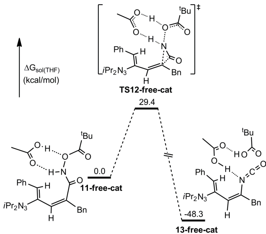
Figure S2 Gibbs free energy profile for the concerted Lossen rearrangement/OPiv migration without rhodium catalyst.
