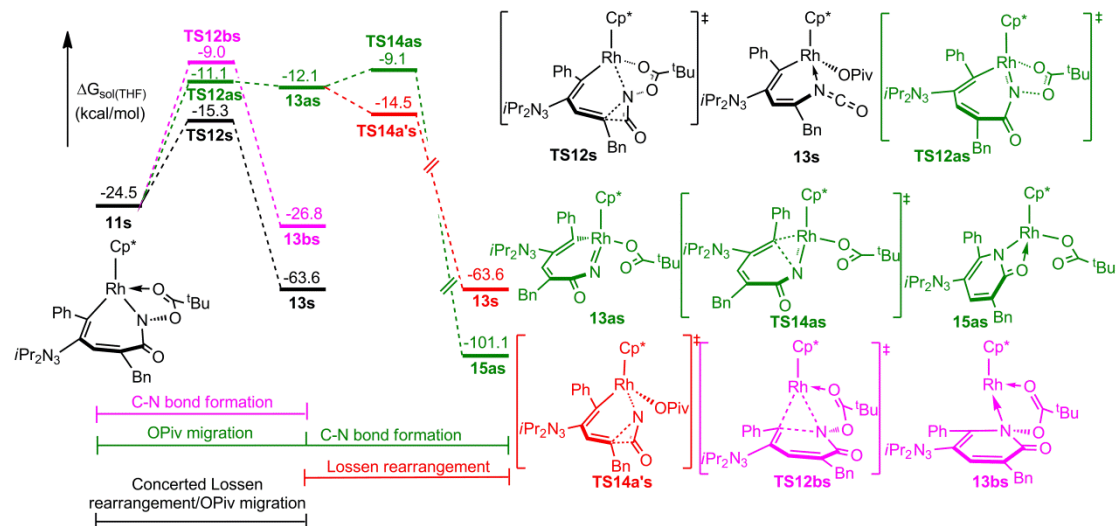
Figure S5 Gibbs free energy profiles for full optimization in tetrahydrofuran of alternative pathways starting from intermediate 11s .
