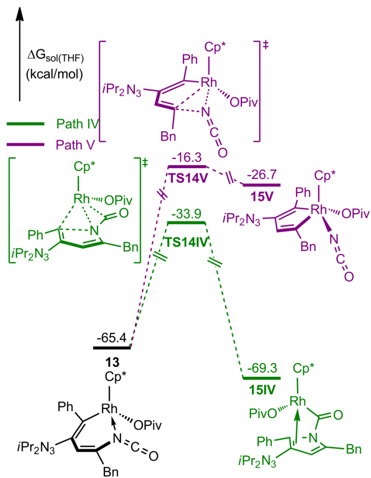
Figure S7 Gibbs free energy profiles for both pathways starting from isocyanate 13 .
