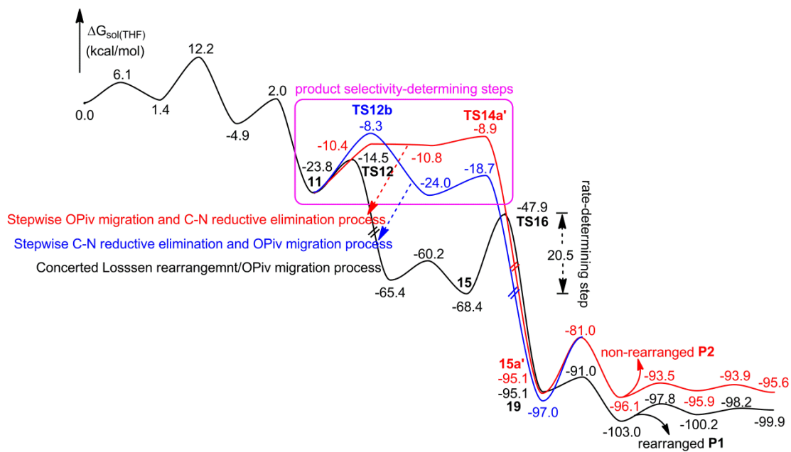
Figure S9 Summary on the free energy profiles for the formation of rearranged and non-rearranged products.
