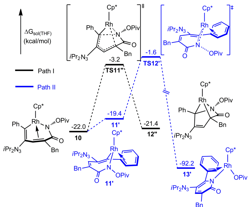
Figure S3 Gibbs free energy profiles of two pathways for C-N reductive elimination starting from 10 .
