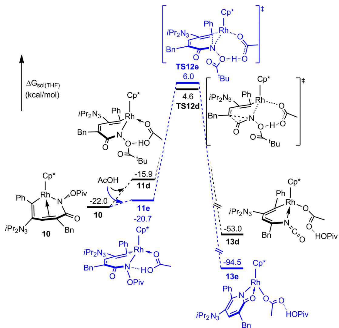
Figure S4 Gibbs free energy profile for the concerted Lossen rearrangement/N-O bond cleavage and C-N bond formation/N-O bond cleavage assisted by AcOH.
