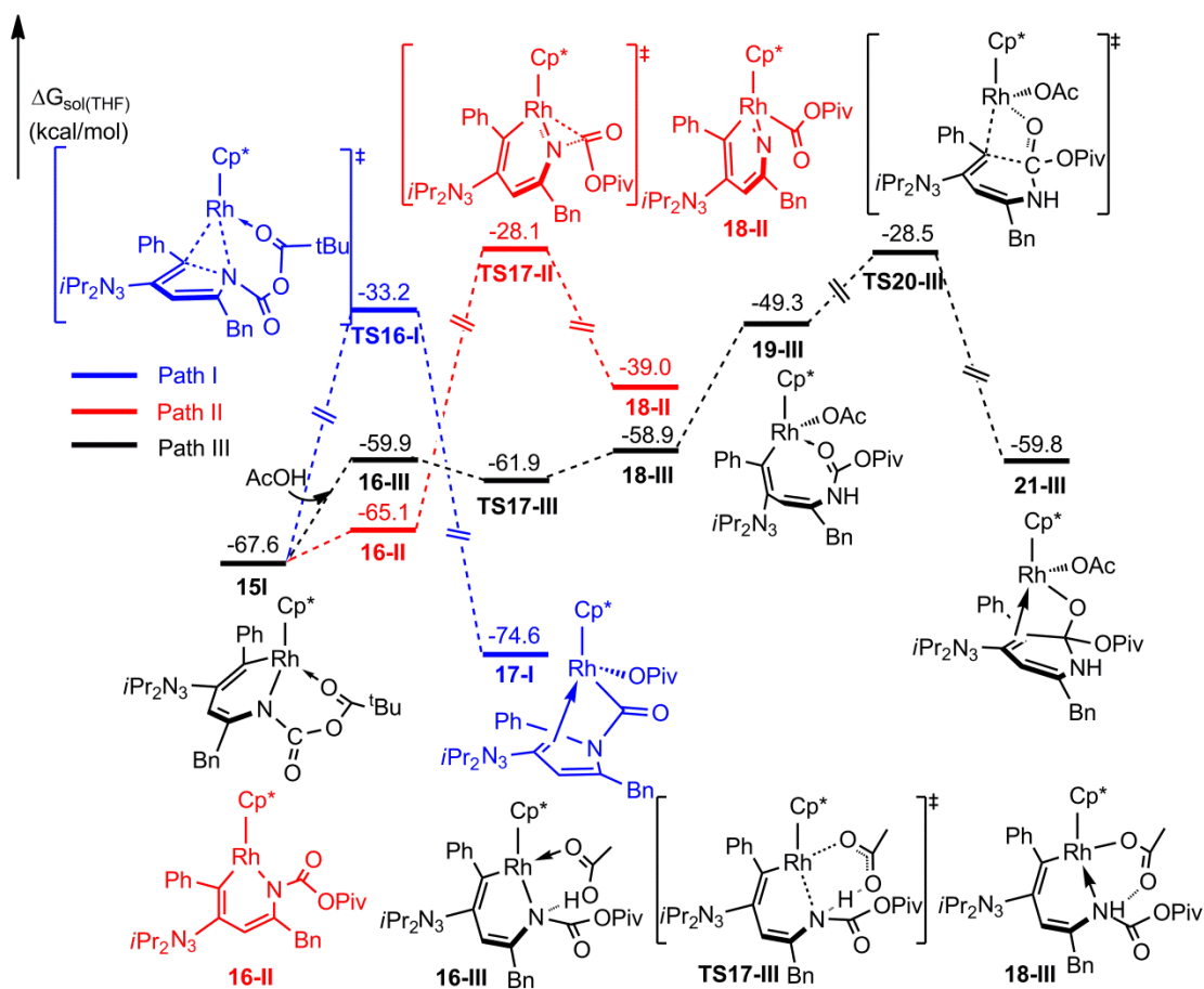
Figure S8 Gibbs free energy profiles for plausible pathways starting from intermediate 15I .
