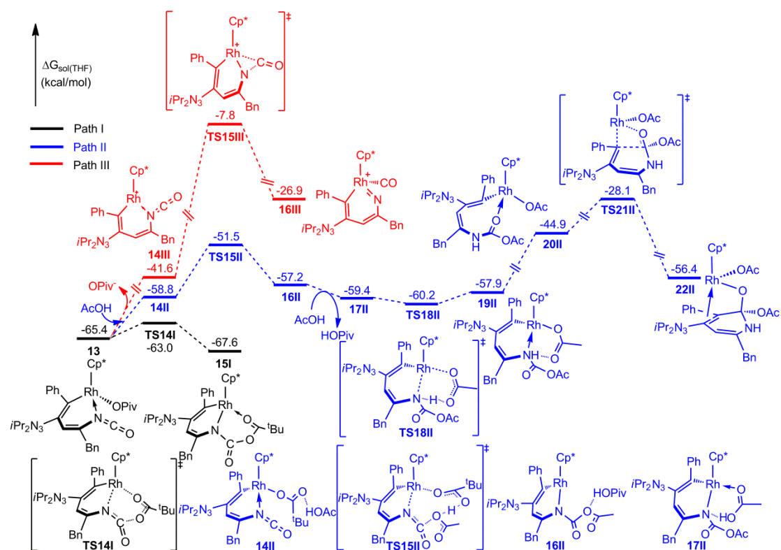
Figure S6 Gibbs free energy profiles for three pathways starting from isocyanate 13 .
