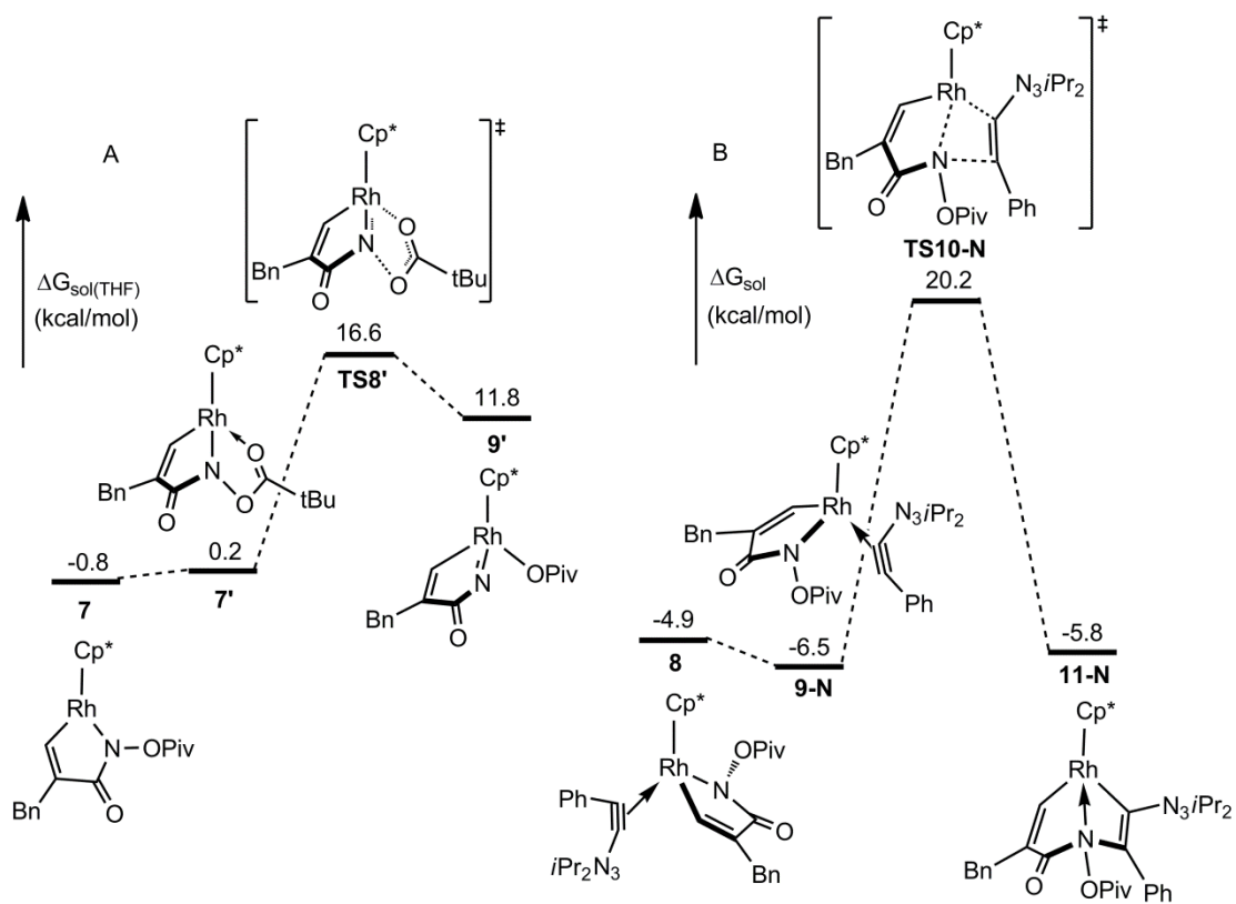
Figure S1 Gibbs free energy profiles for (A) OPiv migration from N to Rh prior to alkynyl insertion, and (B) insertion of alkynyl triazene into Rh-N bond.
