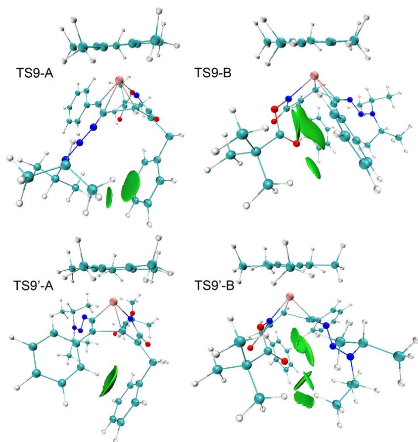
Figure S10 Intramolecular weak interactions a for TS9 and TS9' .
