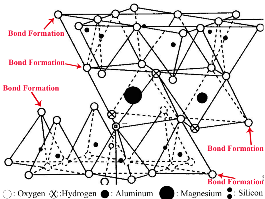
Fig. S2 Bonding sites in exfoliated Mt nanosheets.
