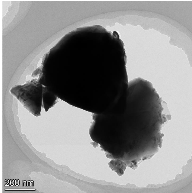
Fig. S2 The bright-field TEM image of BNBTYN-5KN ceramic powder.
