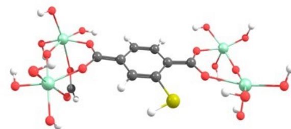
M-SH/S 1
