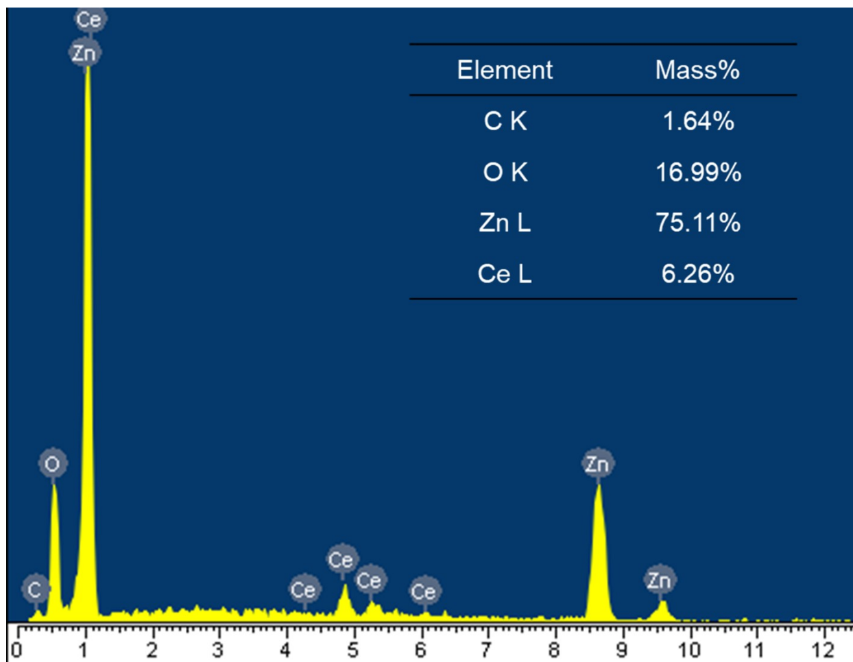
Figure S2. EDX spectra of C/Ce-ZnO materials. Inset tables: Elemental analysis of corresponding materials.
