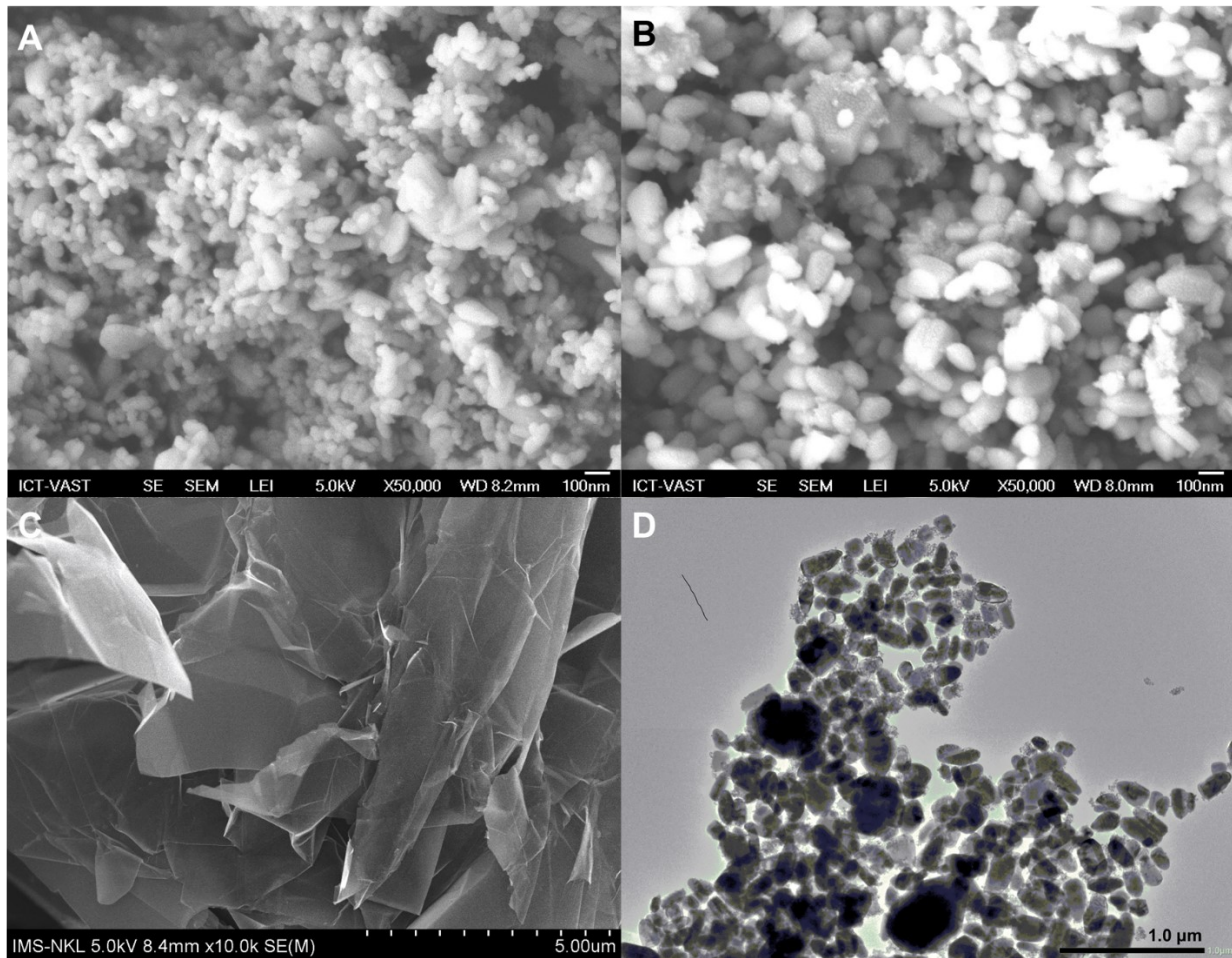
Figure S1. SEM images of (A) ZnO, (B) C/Ce-ZnO, and (C) graphene. (E) HR-TEM image of CCZG.
