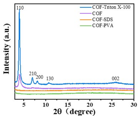
Figure S1. PXRD patterns of COF, COF-Triton X-100, COF-SDS, COF-PVA.
