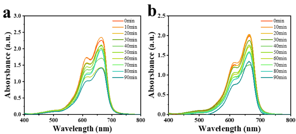
Figure S2. UV-vis absorption spectra of MB solution by COF-SDS (a), COF-PVA (b).
