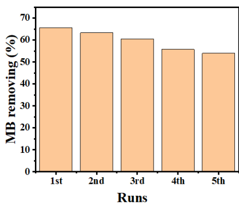
Figure S3. Reusability of COF for the photocatalytic degradation of MB solution.
