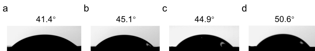
Figure S1 Water contact angles on the surfaces of \text{Ti}_3\text{C}_2\text{T}_x , \text{Ti}_3\text{C}_2\text{T}_x -4h, \text{Ti}_3\text{C}_2\text{T}_x -8h, and \text{Ti}_3\text{C}_2\text{T}_x -12h films.
