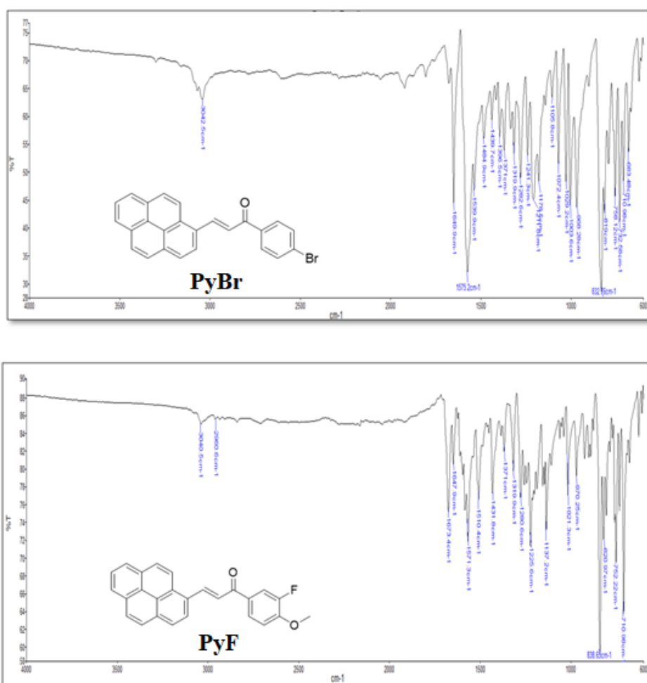
Figure S1. The FTIR spectrum of PyBr and PyF.
