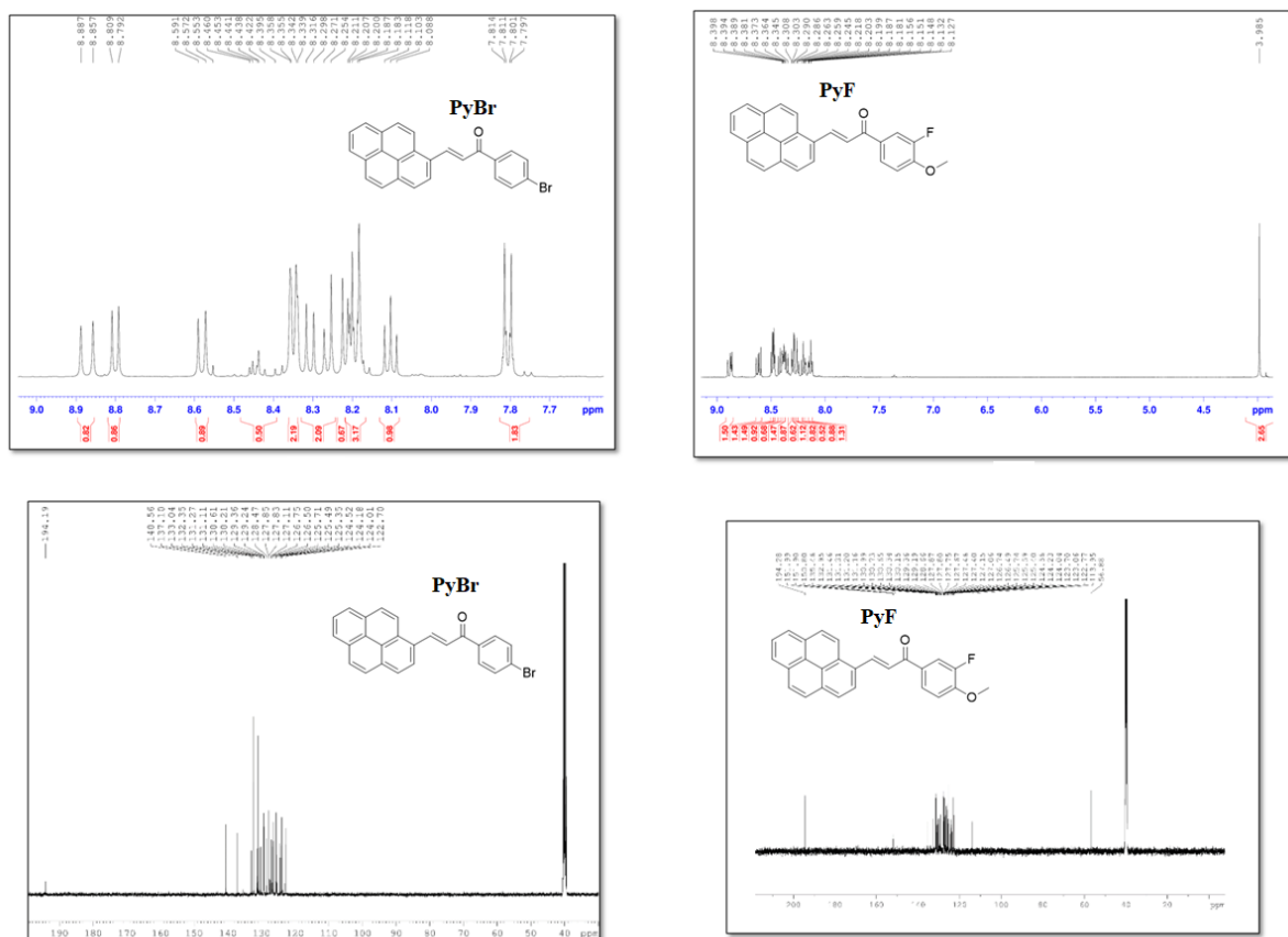
Figure S2. ^1\text{H} and ^{13}\text{C} NMR spectra of PyBr and PyF .
