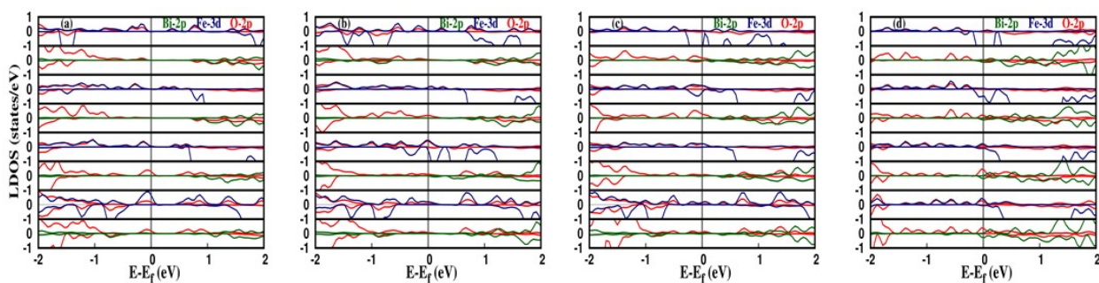
Fig. 11 Local density of states(LDOS) of 8L slab-thicknesses with FeO 2 termination for (a) structure-I, (b) structure-II, (c) structure-III, and (d) structure-IV respectively.
