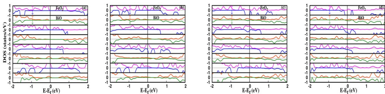
Fig. 10 Density of states (DOS) of 8L slab-thicknesses with FeO 2 termination for (a) structure-I, (b) structure-II, (c) structure-III, and (d) structure-IV respectively.
