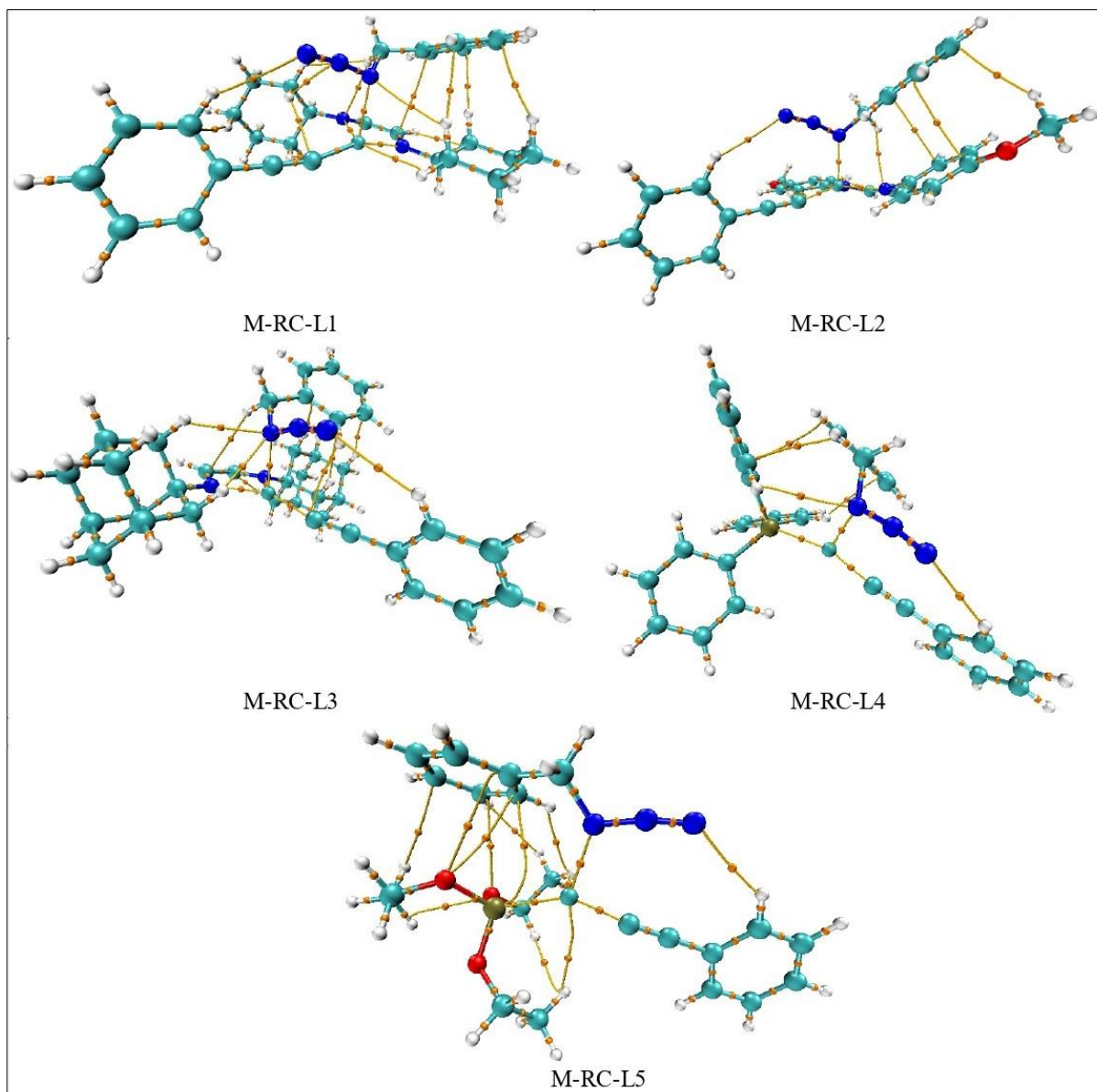
. Fig. S1. AIM of RC (reactive complexes) in the mononuclear pathway calculated at MN12L.
