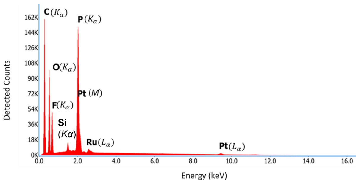
Figure S12: EDX spectrum of HT_non_operated cell shows the presence of C, O, F, P, Pt and Ru.
