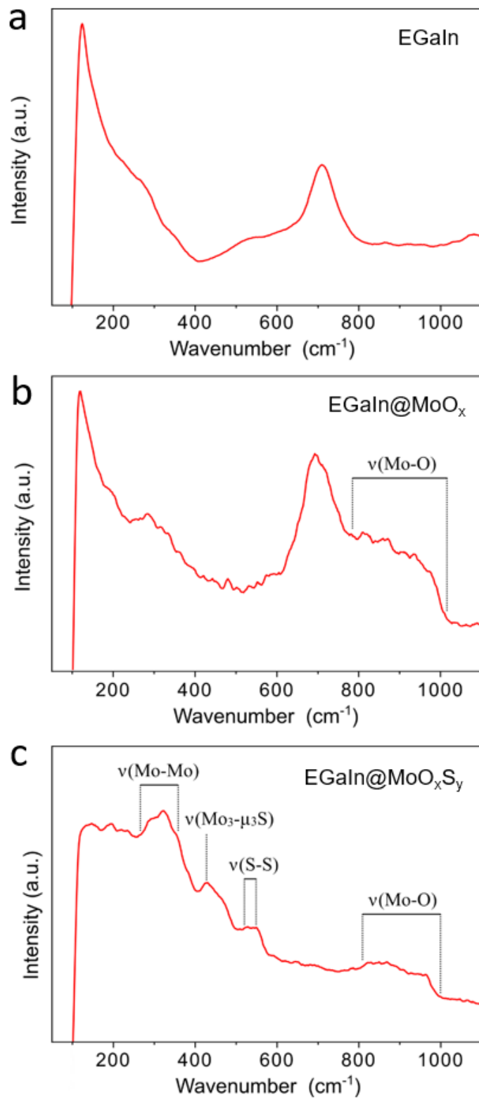
Fig. S2. Raman spectra of a) EGaIn, b) EGaIn@MoO x , and c) EGaIn@MoO x S y microparticles.
