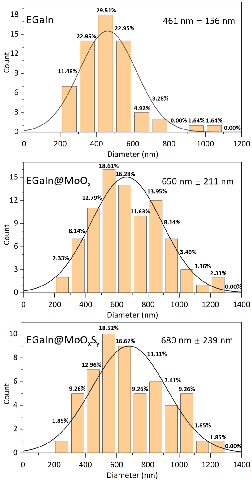
Fig. S1. Size distribution histograms for EGaIn (top), EGaIn@MoO x (middle), and EGaIn@MoO x S y (bottom). The percentage for each size range is marked on the top of each column. The mean and standard deviation values for each material are in the top right corner.
