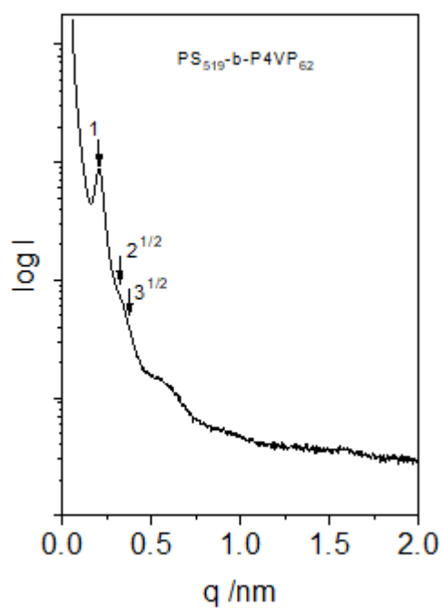
Figure S1: 1D-SAXS profile of self-assembled bulk morphology of PS 519 -P4VP 62 .
