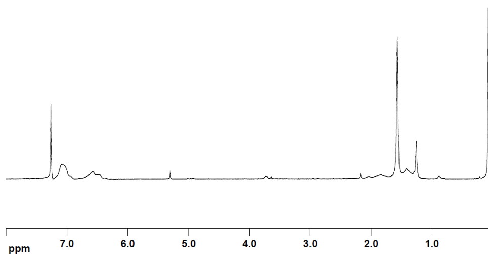
Figure S2: 1 H-NMR spectrum of PS-BuP4VP-Br.
