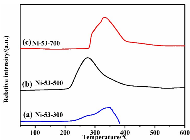
Fig. S2. H 2 -TPR profiles of (a) Ni-53-300, (b) Ni-53-500 and (c) Ni-53-700
