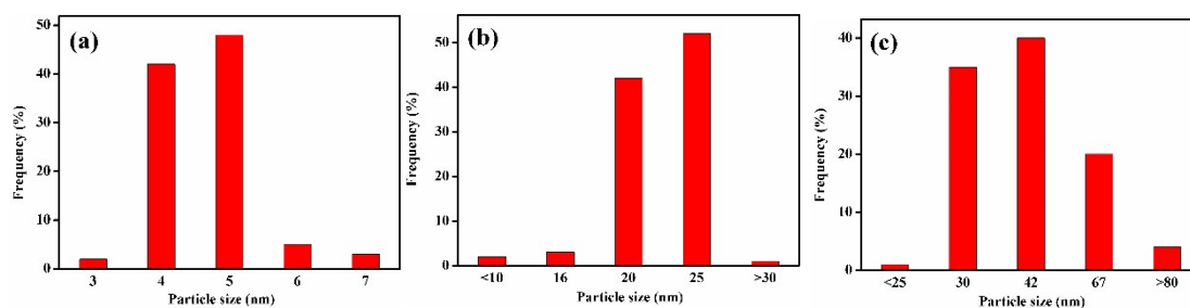
Fig. S1. Ni particle size distribution of (a) Ni-53-300, (b) Ni-53-500 and (c) Ni-53-700
