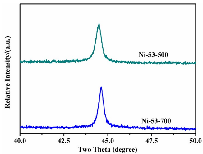
Fig. S3. Ni(111) reflection of Ni-53-500 and Ni-53-700 XRD patterns
