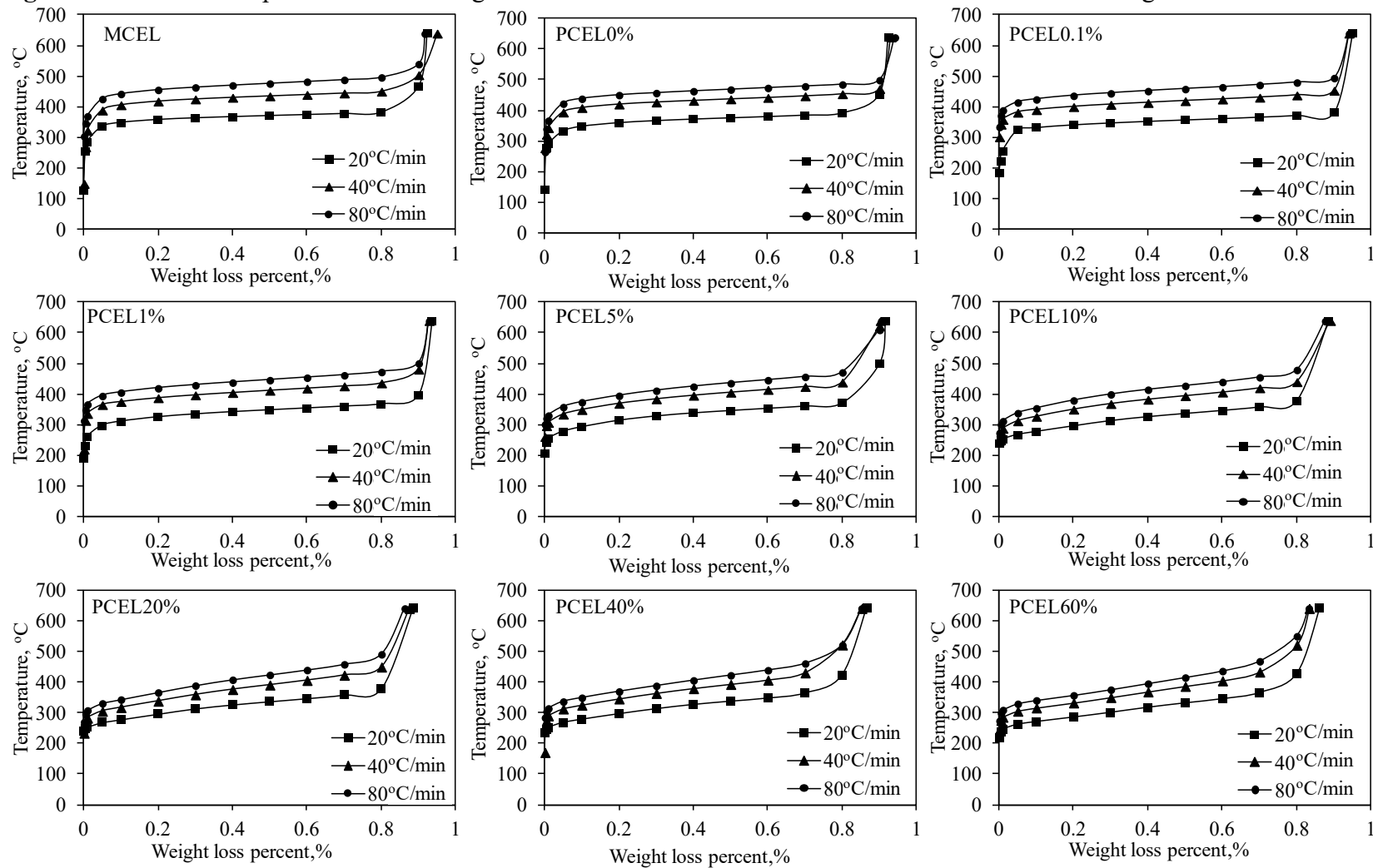
Figure SI3. Plots of temperature vs loss weight of MCEL and PCEL0%-PCEL100% under different heating rate.
