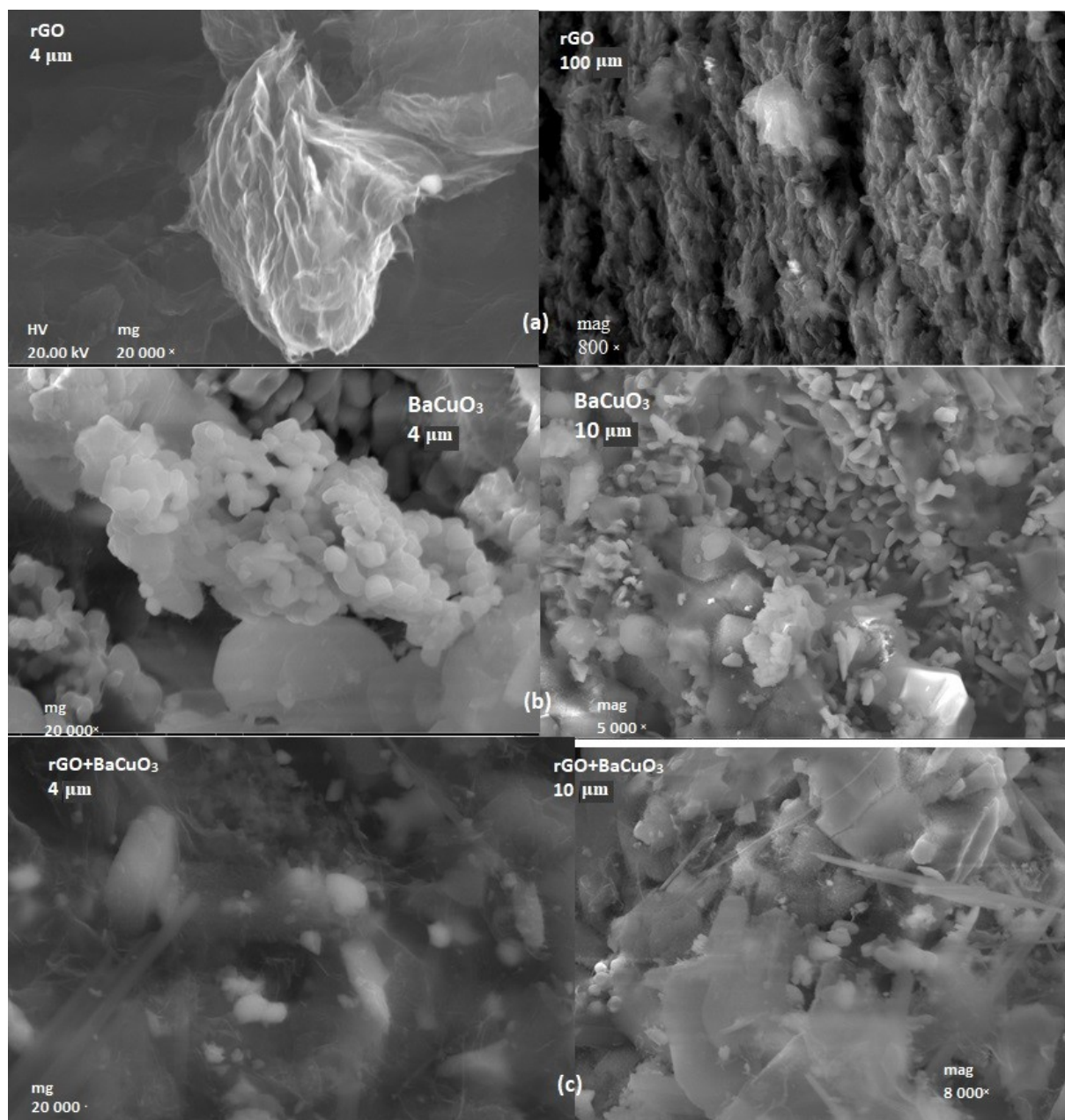
Fig 1S. FEG-SEM micrographs of (a) rGO, (b) BaCuO 3 , and (c) rGO+BaCuO 3 with various magnification.
