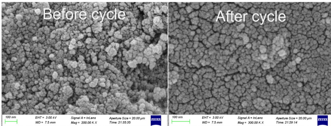
Fig. S2 The FESEM of \text{TiO}_2@\text{Cot} before and after photocatalytic recycling
