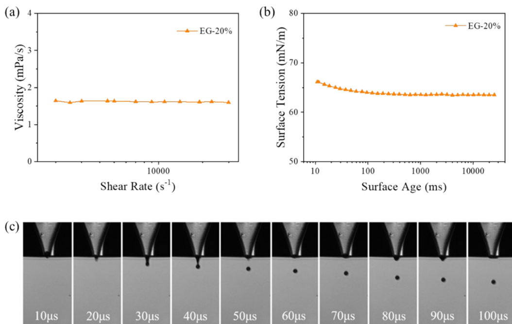
Fig. S1. (a) Viscosity, (b) surface tension and (c) droplet morphology of Reactive Orange 13 ink.
