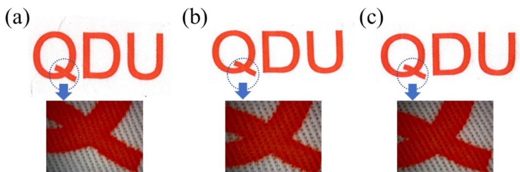
Fig. S3. The outline sharpness of ink-jet printed cotton fabrics treated with alkali: (a) 0 s, (b) 10 s, (c) 60 s.
