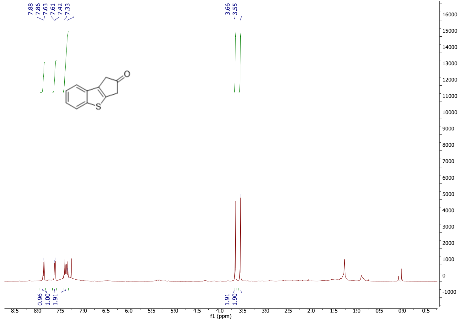
3f: 1,3-dihydro-2H-benzo[b]cyclopenta[d]thiophen-2-one
