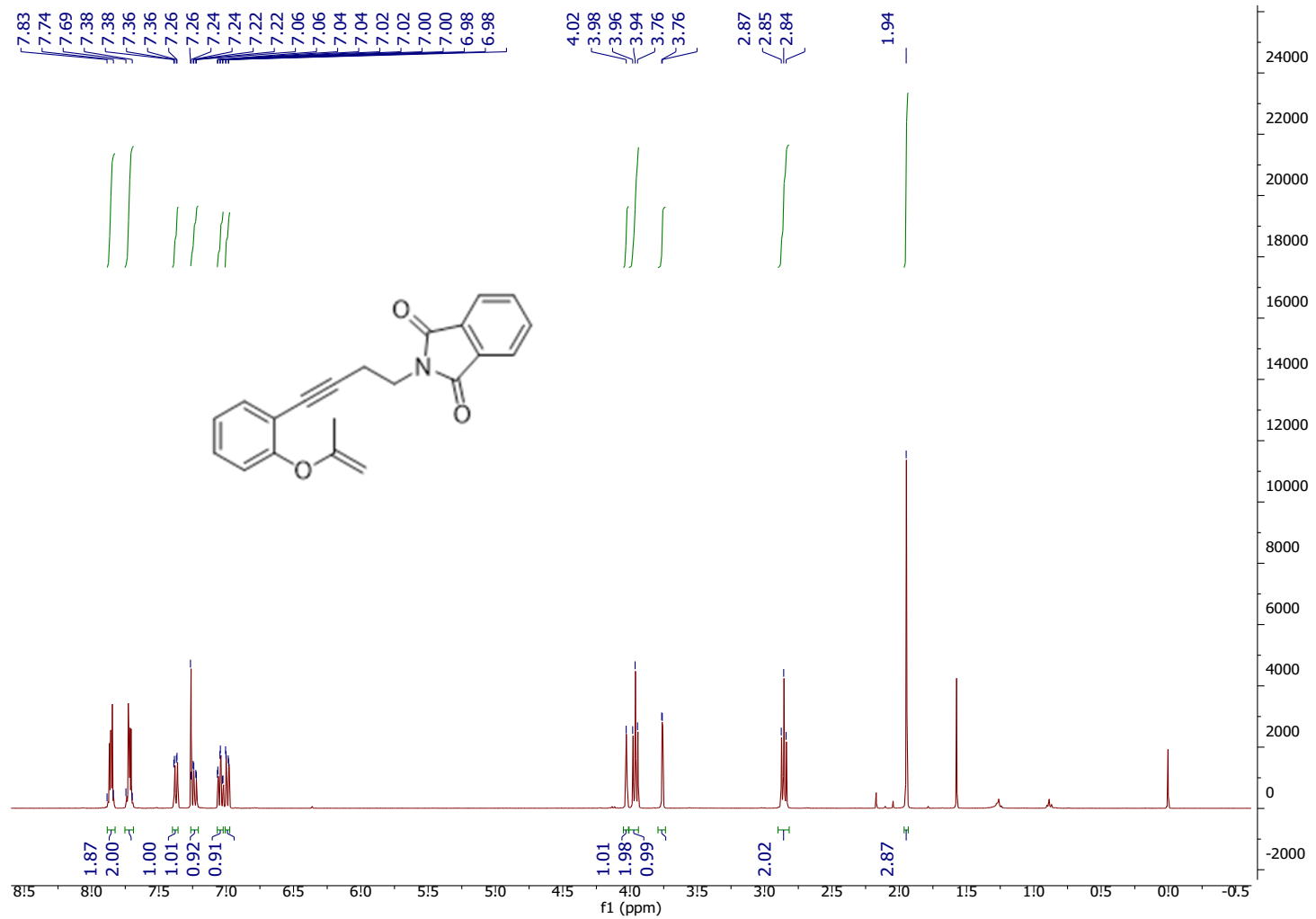
1p: 2-(4-(2-(prop-1-en-2-yloxy)phenyl)but-3-yn-1-yl)isoindoline-1,3-dione
