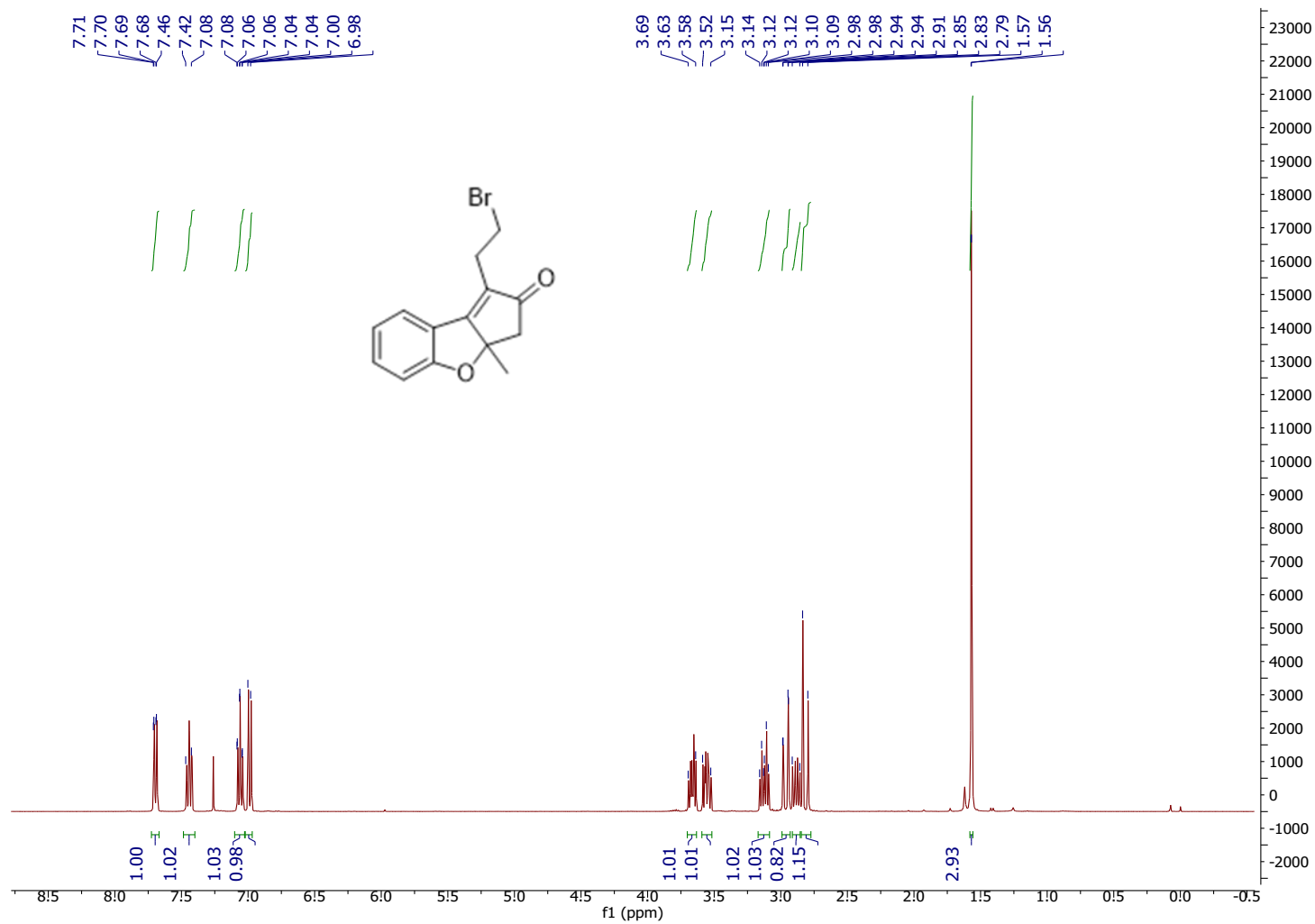
2r: 1-(2-bromoethyl)-3a-methyl-3,3a-dihydro-2H-cyclopenta[b]benzofuran-2-one
