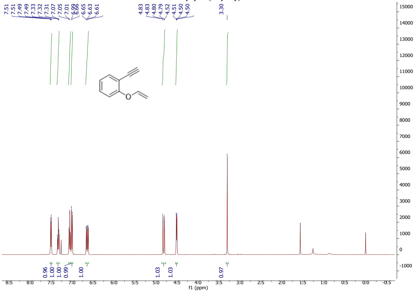
1a: 1-ethynyl-2-(vinylloxy)benzene
