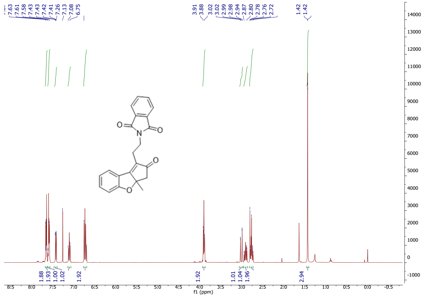
2p: 2-(2-(3a-methyl-2-oxo-3,3a-dihydro-2H-cyclopenta[b]benzofuran-1-yl)ethyl)isoindoline-1,3-dione.
