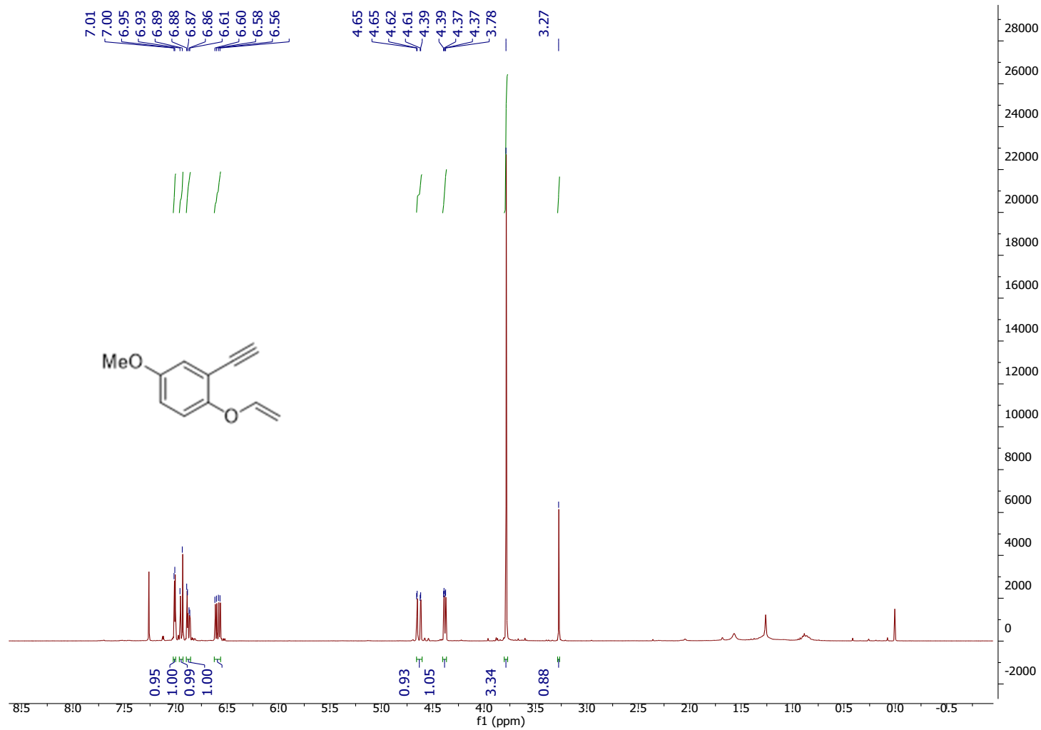
1d: 2-ethynyl-4-methoxy-1-(vinylloxy)benzene
