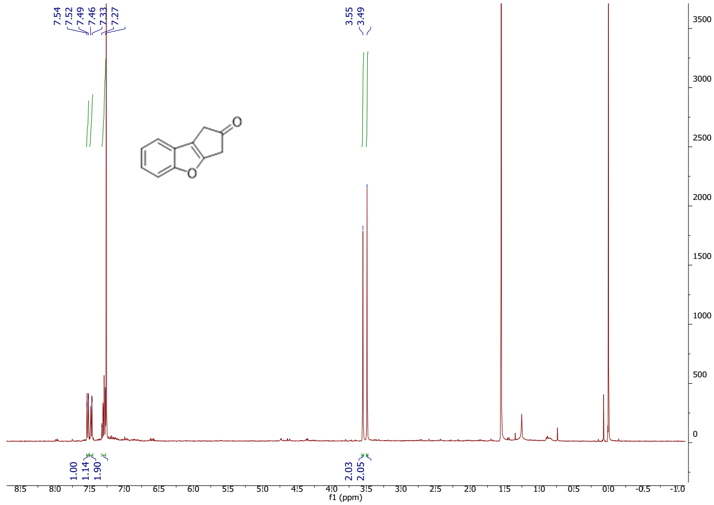
3a: 1,3-dihydro-2H-cyclopenta[b]benzofuran-2-one:
