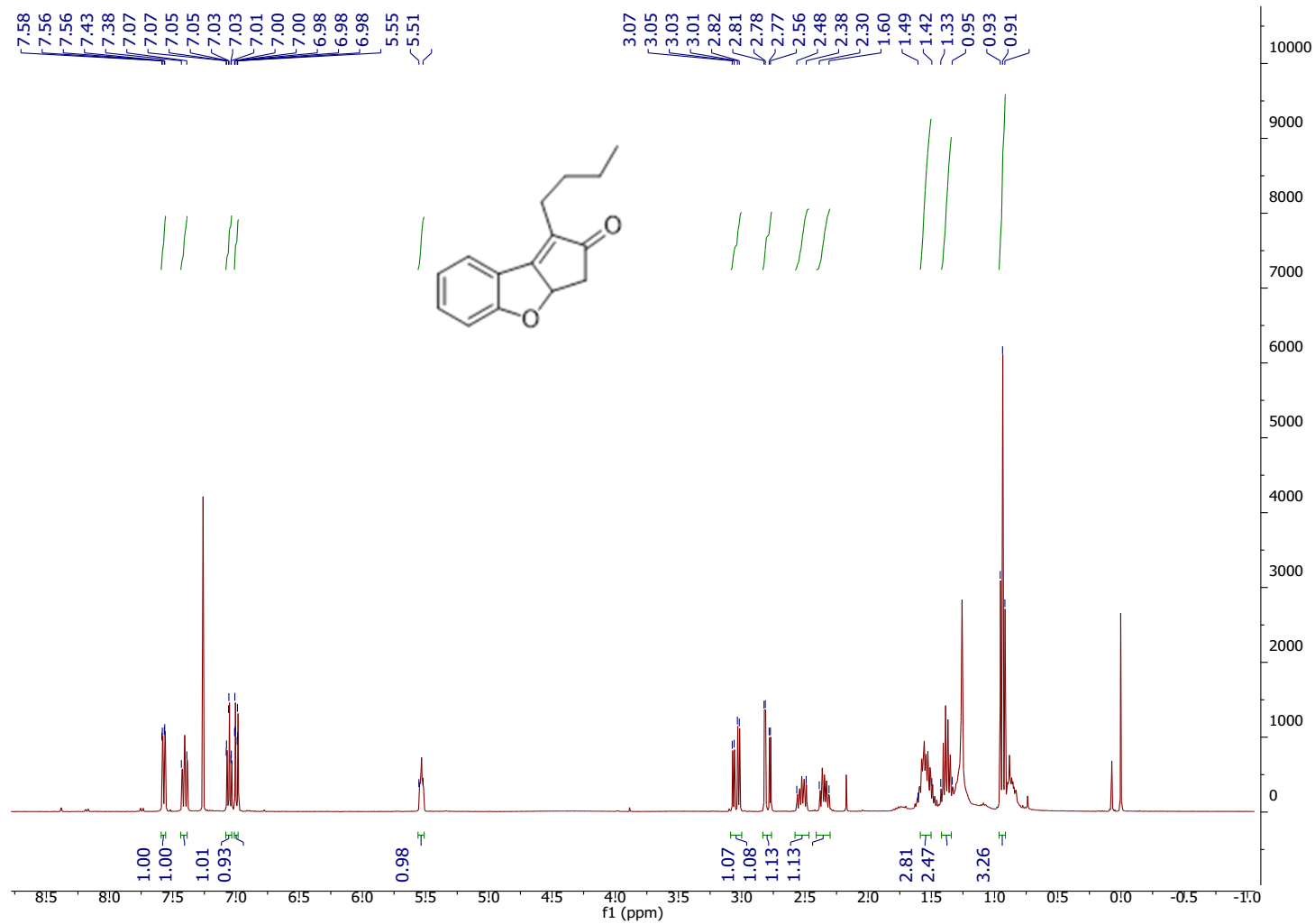
2h: 1-butyl-3,3a-dihydro-2H-cyclopenta[b]benzofuran-2-one.
