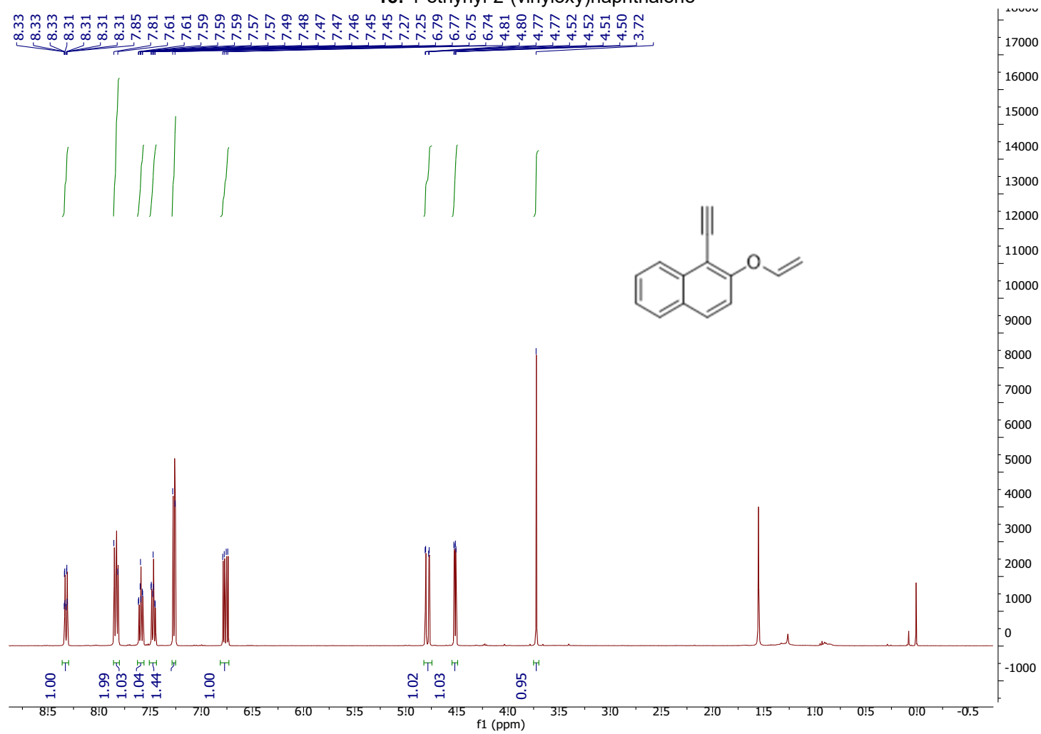
1e: 1-ethynyl-2-(vinyloxy)naphthalene
