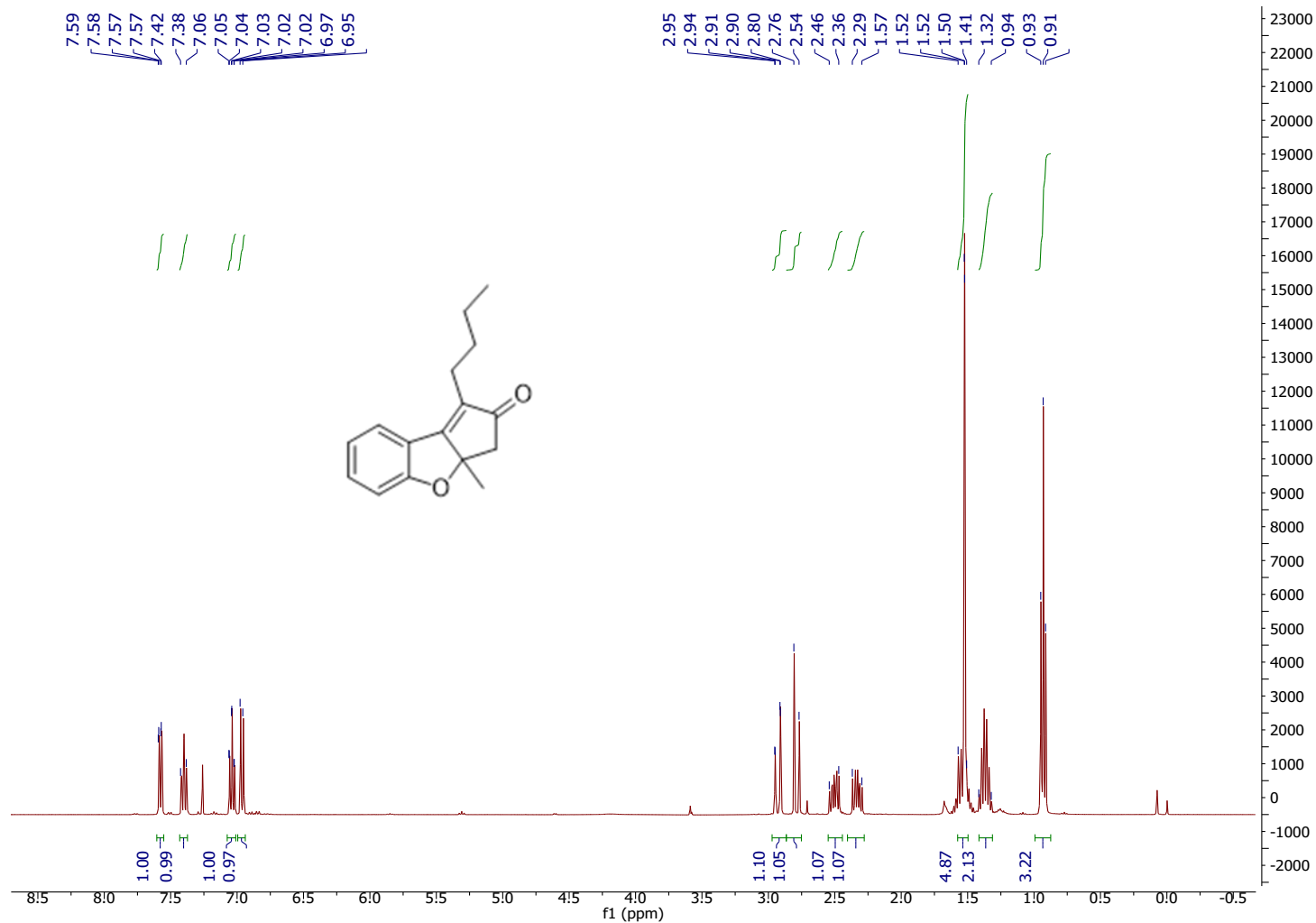
2o: 1-butyl-3a-methyl-3,3a-dihydro-2H-cyclopenta[b]benzofuran-2-one.
