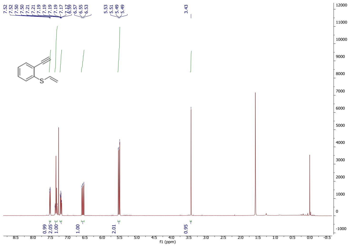
1f: (2-ethynylphenyl)(vinyl)sulfane
