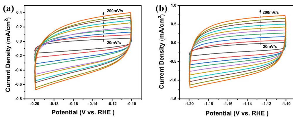
Fig. S1. Cyclic voltammograms of 3D RGO at a scan rate of 20-200 mV s -1 (a) in 0.5 M H 2 SO 4 , (b) in 1 M KOH.
