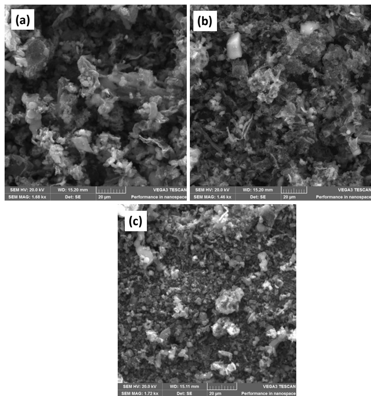
Figure S1: SEM image of (a) HHPB11650_60 (b) HHPB11700_60 (c) HHPB11750_60
