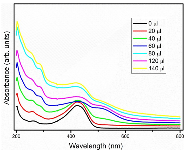
Figure S6: UV-Vis spectra of rGO-CM solution with serial addition of 1,4-dioxane
