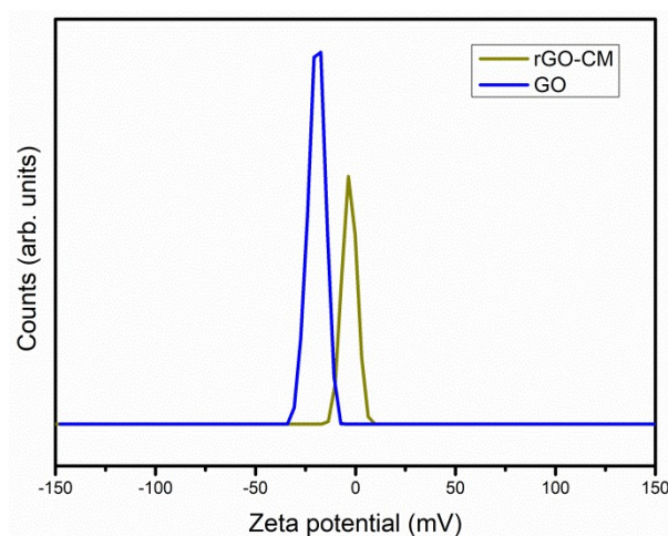
Figure S3: Zeta potential distributions of GO and rGO-CM
