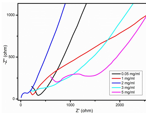
Figure S4: Nyquist plots of rGO-CM (synthesized with different curcumin concentrations) modified electrodes
