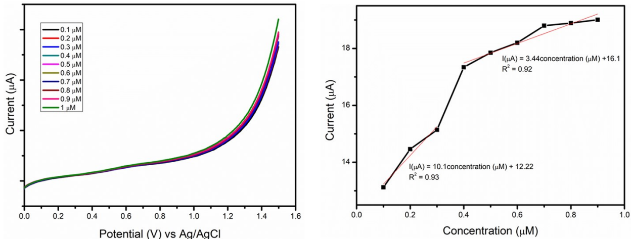
Figure S9: (a) Linear sweep voltammograms of rGO-CM/GCE in increasing concentration (0.1-1 μM) of 1,4-dioxane and (b) the corresponding calibration curve with the red line indicating the best linear fit.
