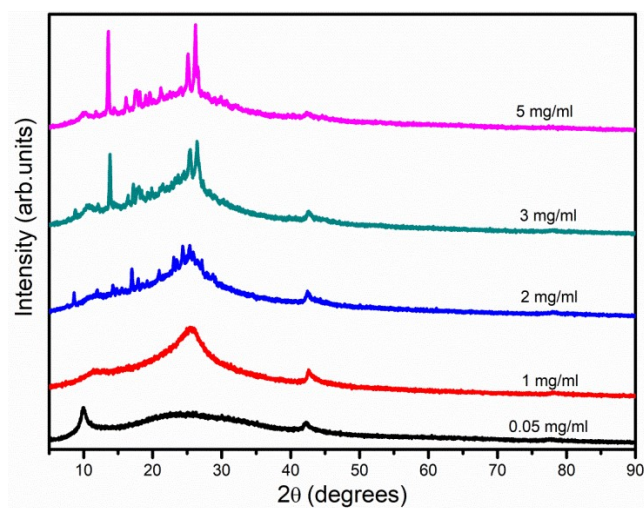
Figure S1: XRD patterns of rGO-CM synthesized with different curcumin concentrations
