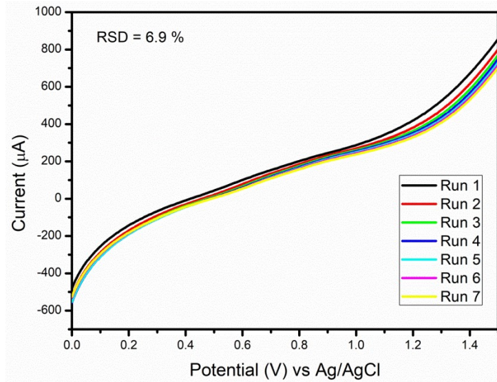
Figure S11: Stability of the current response of the rGO-CM/GCE sensor over seven consecutive runs
