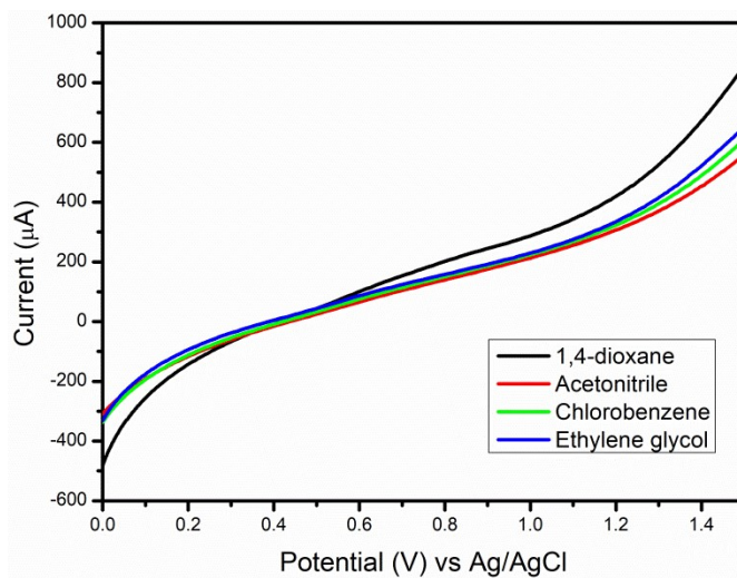
Figure S10: LSV of rGO-CM/GCE in dioxane and other interferants
