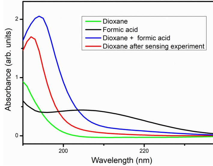
Figure S7: UV-Vis spectroscopy for the identification of the oxidation products
