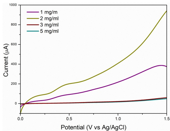
Figure S5: Linear sweep voltammograms of rGO-CM (synthesized with different curcumin concentrations) modified glassy carbon electrode in 15 mM dioxane.
