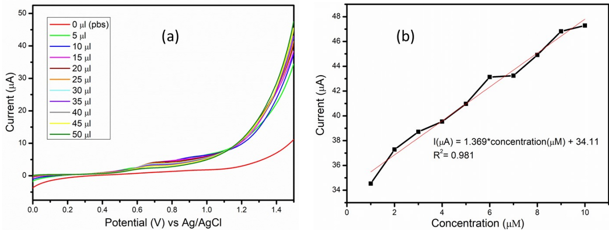
Figure S8: (a) Linear sweep voltammograms of rGO-CM/GCE in increasing concentration (1-10 μM) of 1,4-dioxane and (b) the corresponding calibration curve with the red line indicating the best linear fit.
