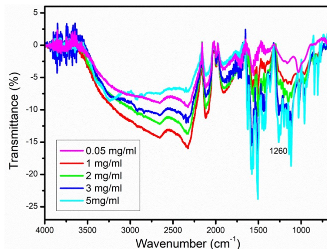
Figure S2: FTIR spectra of rGO-CM samples synthesized with different curcumin concentrations
