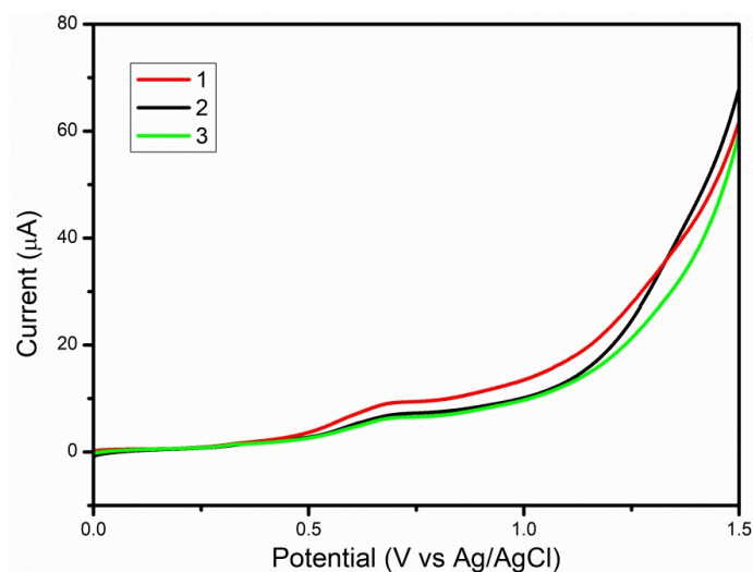
Figure S13: LSV of the rGO-CM coated on different GCEs
