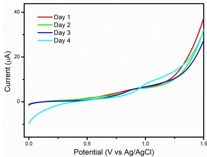
Figure S12: Stability of the rGO-CM/GCE sensor performance towards dioxane detection on different days
