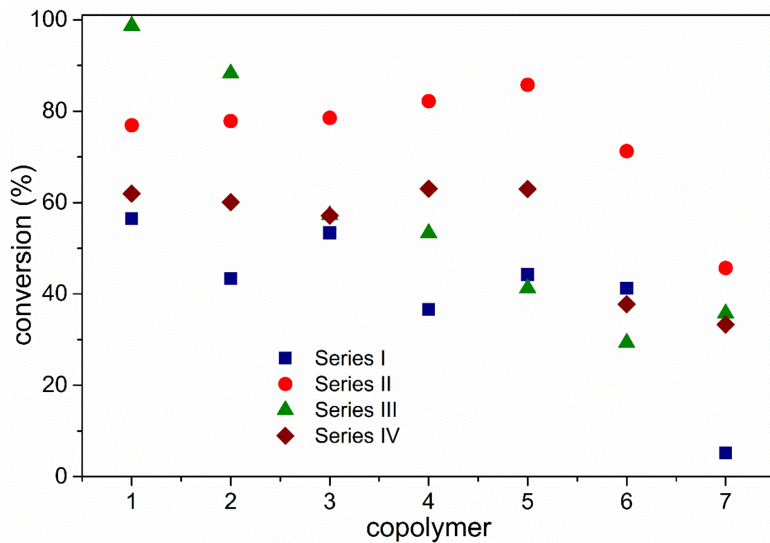
Figure S2. Determination of global conversion in copolymer series I-IV.
