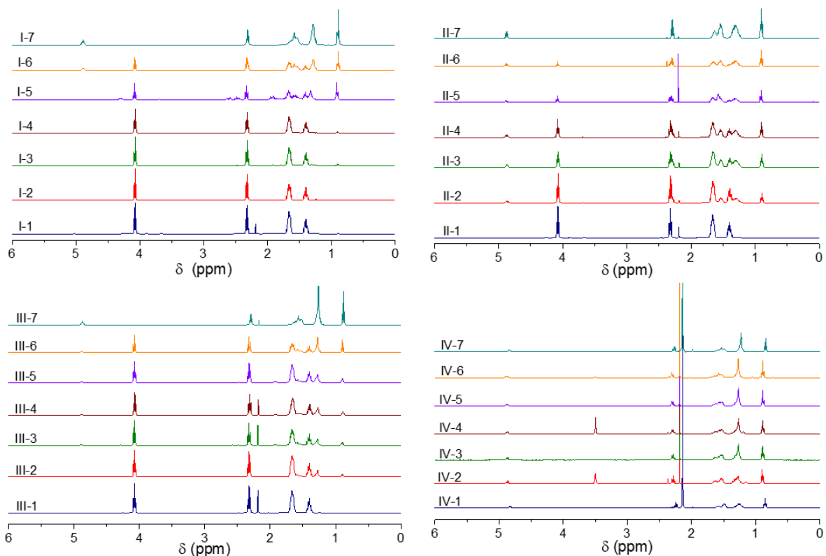
Figure S1. 1 H NMR spectra in copolymer series I-IV.
