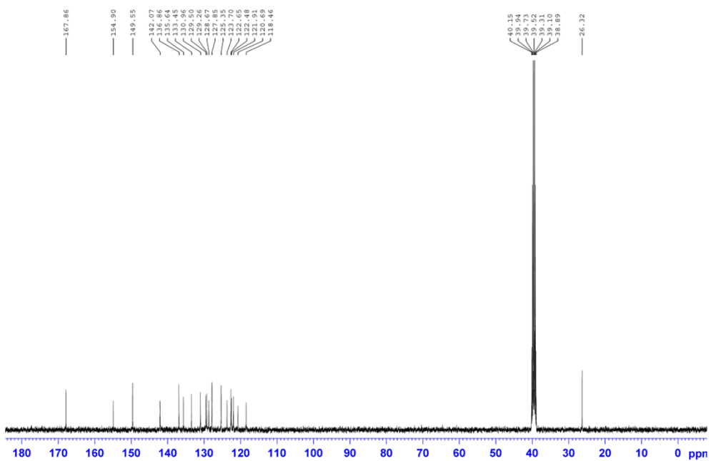
Supplementary Figure.2 13 C NMR spectrum of Se-axitinib
