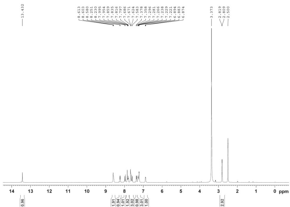
Supplementary Figure.1 1 H NMR spectrum of Se-axitinib
