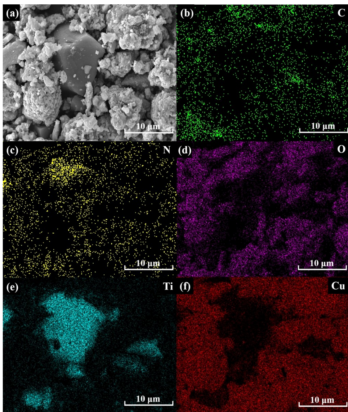
Fig. S 1. (a) SEM image of g-C 3 N 4 /TiO 2 /CuO and elemental mapping of (b) C, (c) N, (d) O, (e) Ti, and (f)
