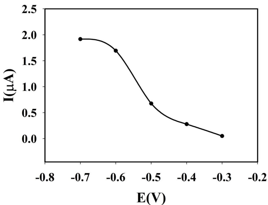
Fig. S1 Effect of the applied potential on the response current of aptasensor when the concentration of \text{H}_2\text{O}_2 was 0.1 \text{mmol/L} in 0.2 \text{mol/L} Tris acetic acid buffer solution (pH 7.0)
