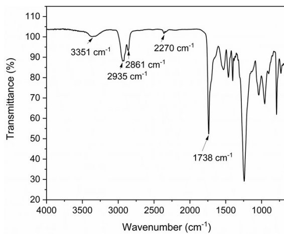
Figure S1 Infrared spectra of WPU prepolymer.
