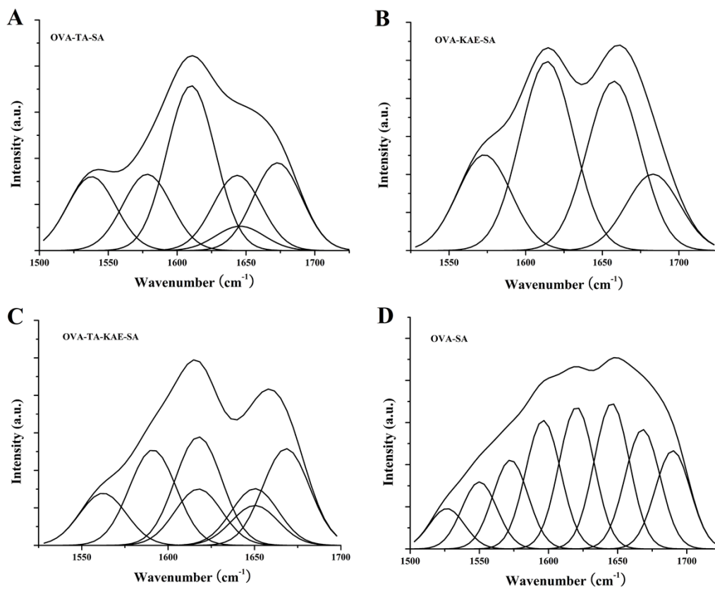
Supplementary Fig. S2 Segregated and iterative curve-fitted Raman bands in amide I region.
