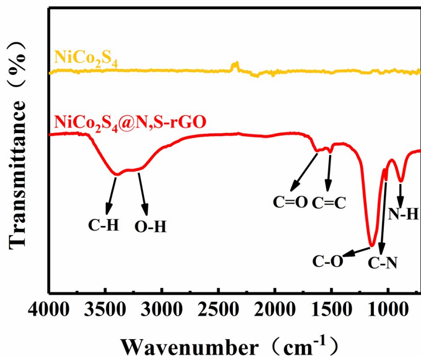
Fig. S1. FT-IR spectra of the \text{NiCo}_2\text{S}_4 and \text{NiCo}_2\text{S}_4@\text{N,S-rGO}
