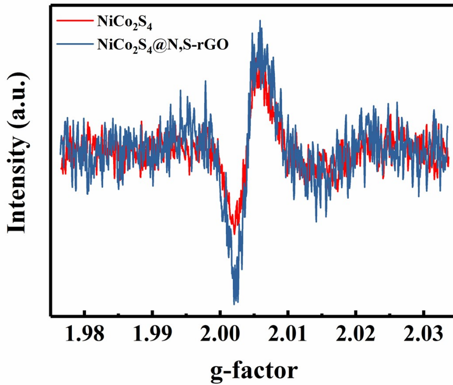
Fig. S3. EPR spectra of the \text{NiCo}_2\text{S}_4@\text{N,S-rGO} and \text{NiCo}_2\text{S}_4
