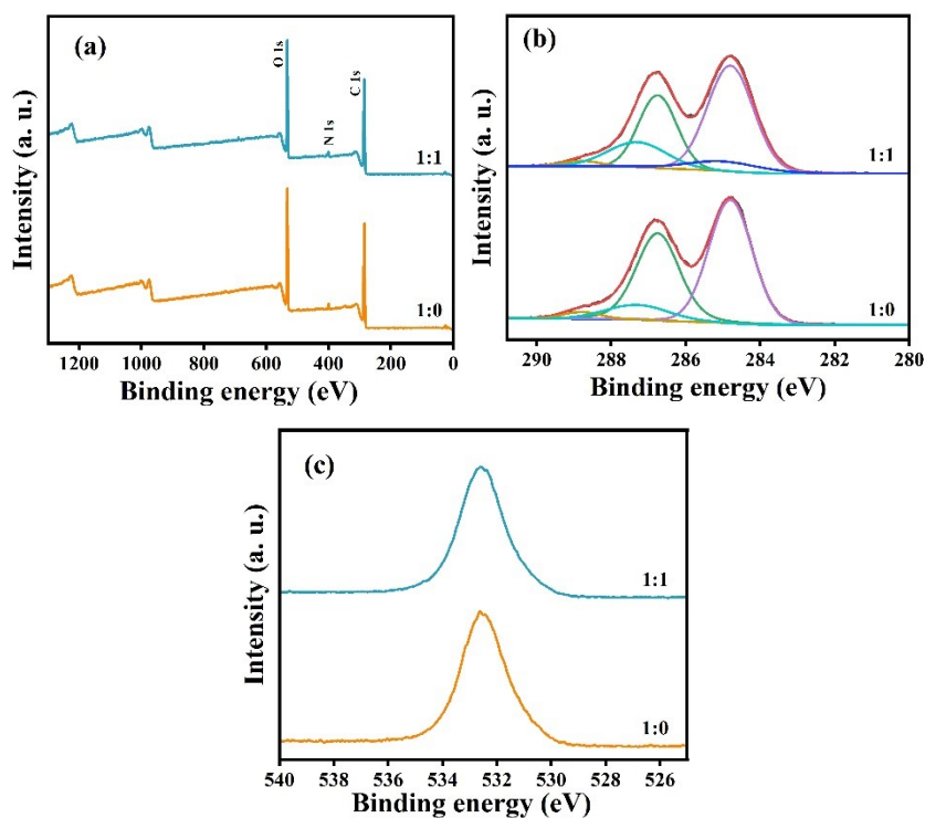
Fig.S3 XPS spectra of modified GO membranes: (a) full spectra; (b) C1s core level spectra; (c) O1s C1s core level spectra.
