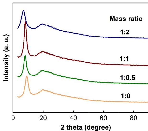
Fig.S4 XRD patterns in an intensive range of modified GO membranes with different ratios of GO to NDT.
