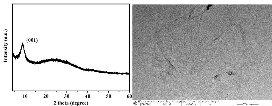
Fig. S1 XRD and TEM images of the as-prepared GO sheets
