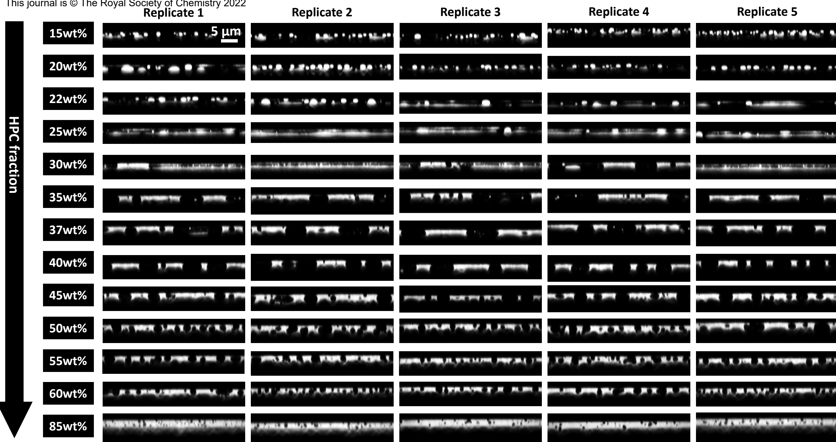
ESI 1. CLSM micrograph replicates of the cross-sectional structures of the EC/HPC films for the 13 EC/HPC ratio one week after spinning. The bright phase is HPC, and the dark phase is EC. Air surface is towards the bottom and the substrate is towards the top in each cross section. This Figure is supplementary information to Figure 9b.
