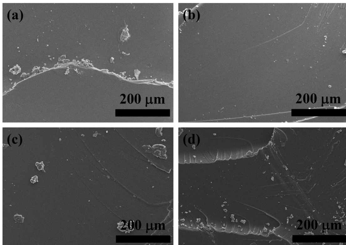
Fig. S1 SEM images of tung oil-based epoxy resins curing with different curing agents after tensile tests: (a) TODGE-MHHPA, (b) TODGE-DDM, (c) TOTGE-MPD, and (d) TOTGE-DDM.
