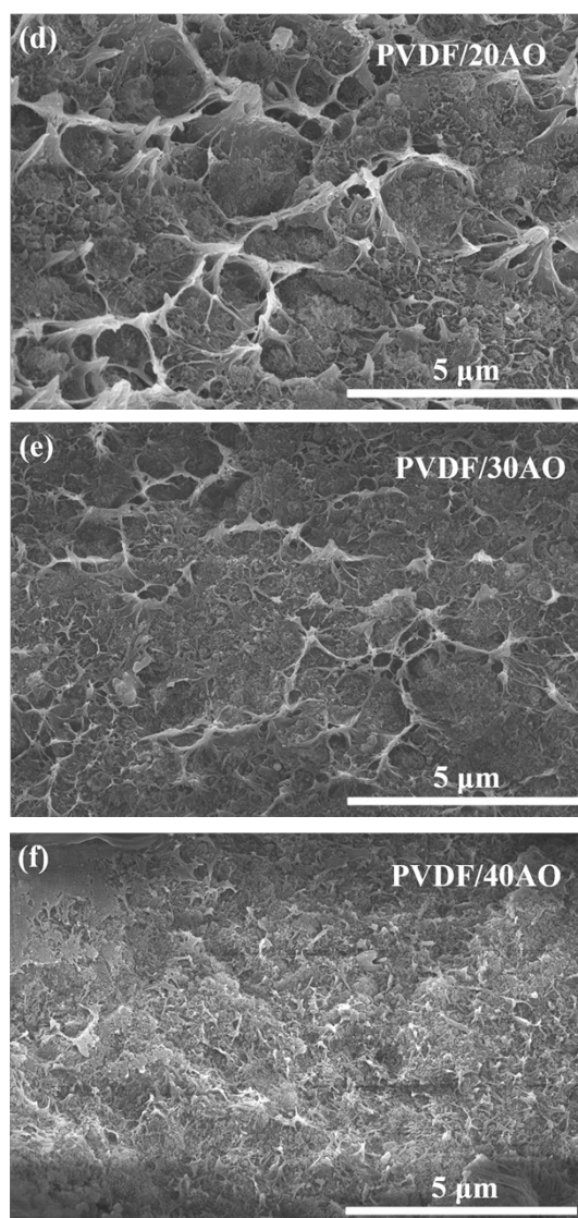
Figure S1. (a) TEM image of AO. SEM images of (b) pristine PVDF film, (c) PVDF/10AO composite film, (d) PVDF/20AO composite film, (e) PVDF/30AO composite film, (f) PVDF/40AO composite film.
