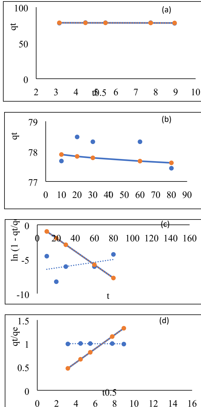
Figure (3): kinetic model adsorption on AgNP/Go/Chitosan for Mn ions (a) linear intraparticle diffusion, (b) nonlinear intraparticle diffusion, (c) Pore diffusion (d) film diffusion.
