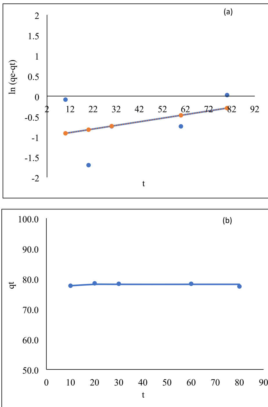
Figure (1): Adsorption on AgNP/Go/Chitosan in pseudo-first-order of Mn ions by (a) linear analysis, (b) nonlinear analysis
