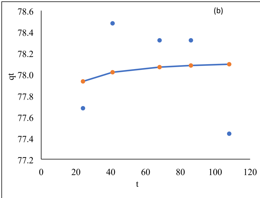
Figure (2): Adsorption on AgNP/Go/Chitosan in pseudo-second-order of Mn ions by (a) linear analysis, (b) nonlinear analysis
