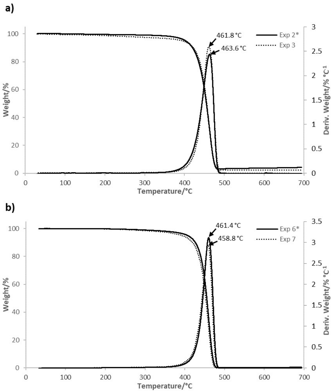
Figure S2. TGA thermograms of the copolymers obtained with a) metallocene and b)
