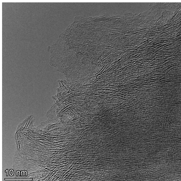
Fig.S3 TEM image of MoS 2 -CA(0.02)
