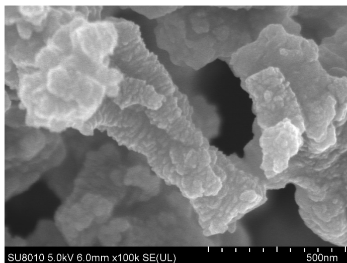
Fig.S2 SEM image of MoS 2 -CA(0.03)
