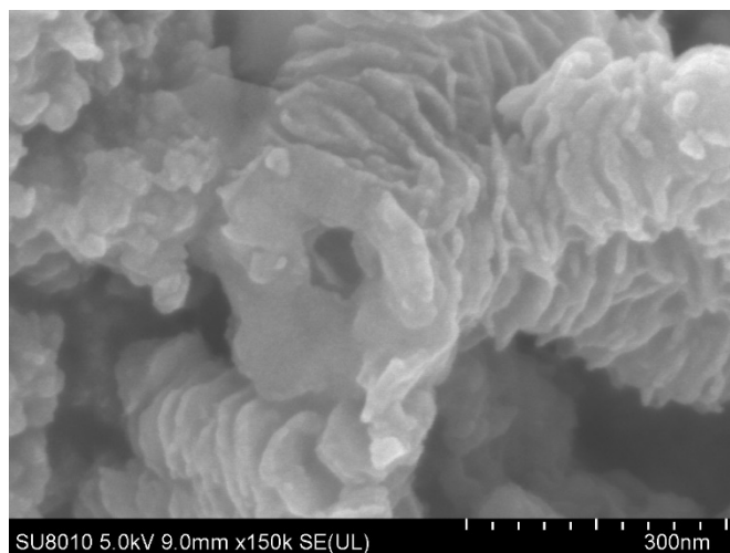
Fig.S1 SEM image of MoS 2 -CA(0.02) with hole
