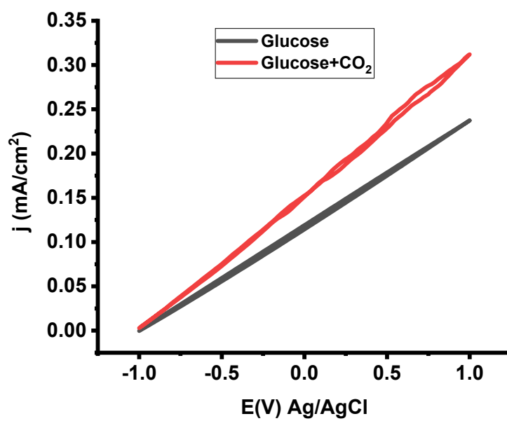
Supplementary Figure 1; Electrolysis using different electrolytes
