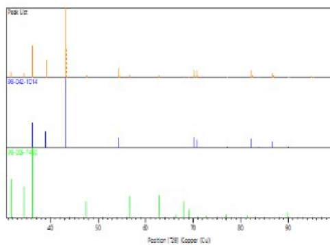
Supplementary Figure 2; XRD results
