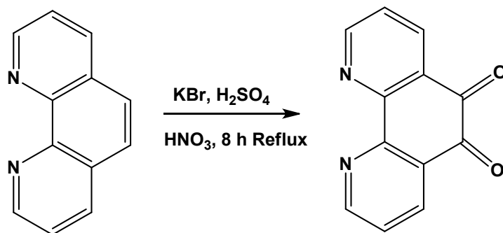
Scheme S1 ‡ - Preparation of 1,10-phenanthroline 5,6-dione
