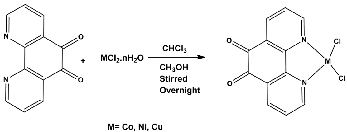
Scheme S2 \ddagger - Syntheses of [M(Phen-dione)]
