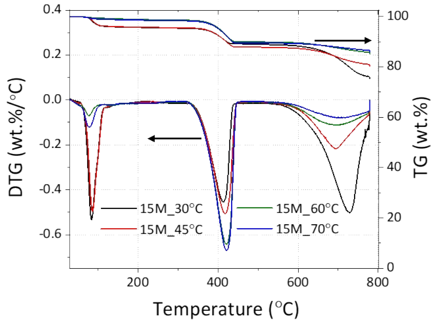
SEI_III: TG/DTG trends registered for the samples reacted at 30, 45, 60, and 70°C in 15M NaOH solutions.
