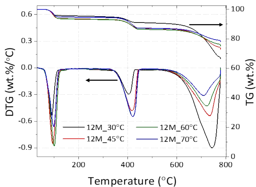
SEI_II: TG/DTG trends registered for the samples reacted at 30, 45, 60, and 70°C in 12M NaOH solutions.
