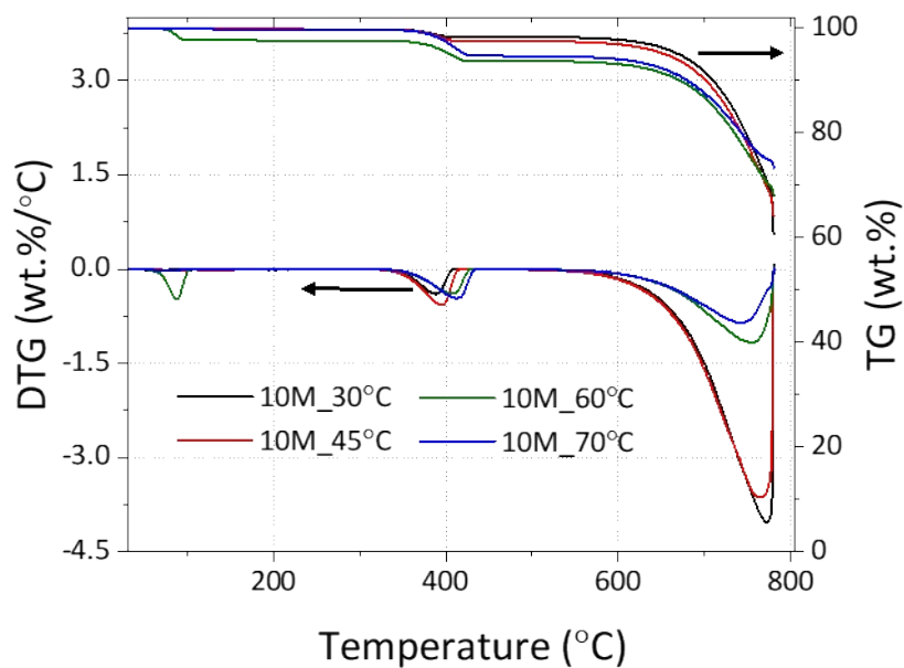
SEI_I: TG/DTG trends registered for the samples reacted at 30, 45, 60, and 70°C in 10M NaOH solutions.
