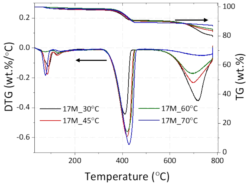
SEI_IV: TG/DTG trends registered for the samples reacted at 30, 45, 60, and 70°C in 17M NaOH solutions.
