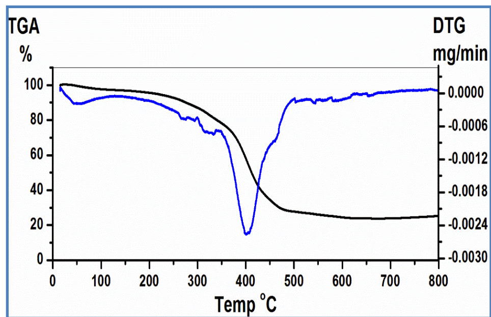
Fig. S2. TGA curve of Sm (III) nanocomplex
