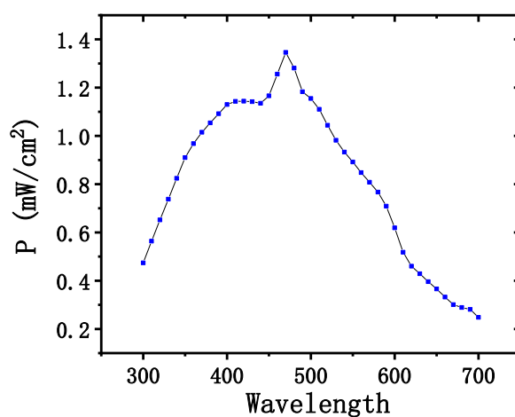
Fig. S2: Light intensity distribution plot curve.
