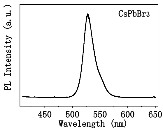
Fig. S1: PL profiles of the CsPbBr 3 particle
