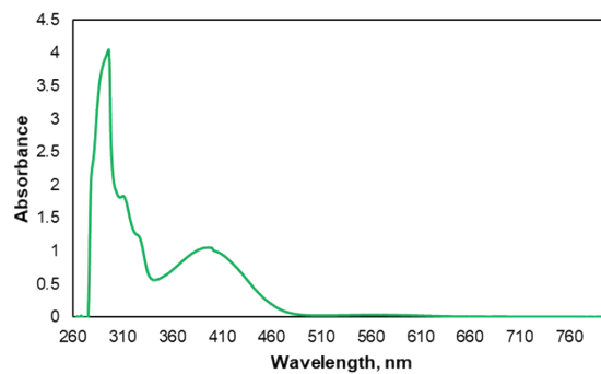
Fig. S6 UV-Vis spectrum of Fe 3 O 4 @SiO 2 -APTES-Fe 2 L DAR in benzoxazole synthesis
