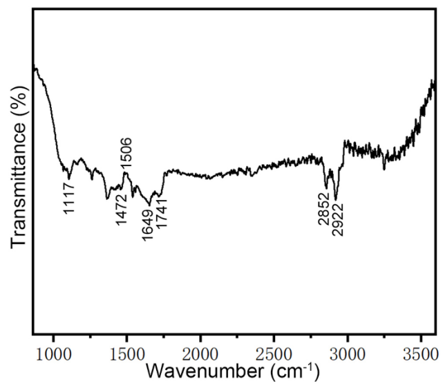
Fig. S3. FTIR spectrum of pure AgBr
