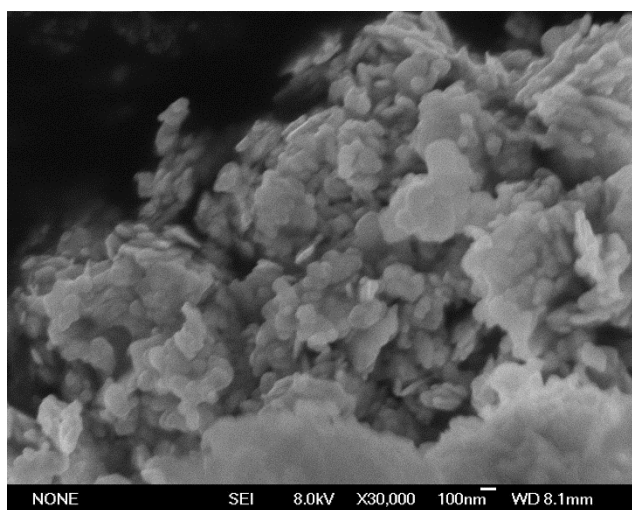
Fig. S2. SEM image of BBN nanosheets
