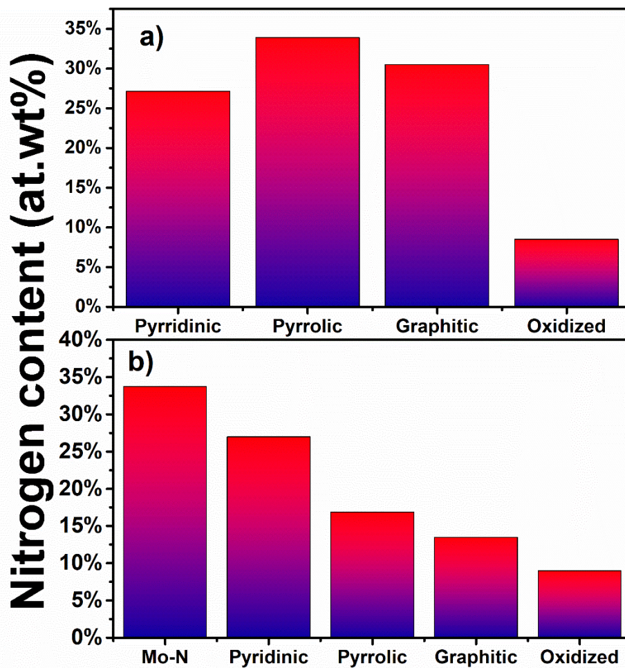
Figure S4: The contents of different types of nitrogen in the a) CDNPs and b) POM@CDNPs.
