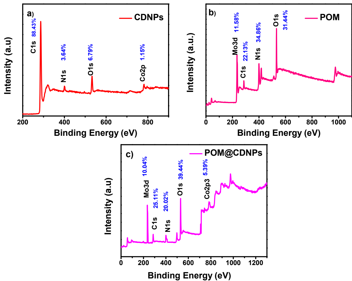
Figure S3: XPS survey spectrum of the CDNPs, POM and POM@CDNPs.
