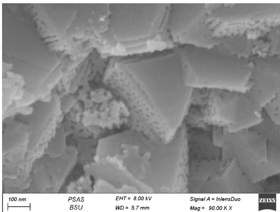
Figure S1: FESEM image for POM@CDNPs where the porous structure of the POM pyramidal shapes is shown.
