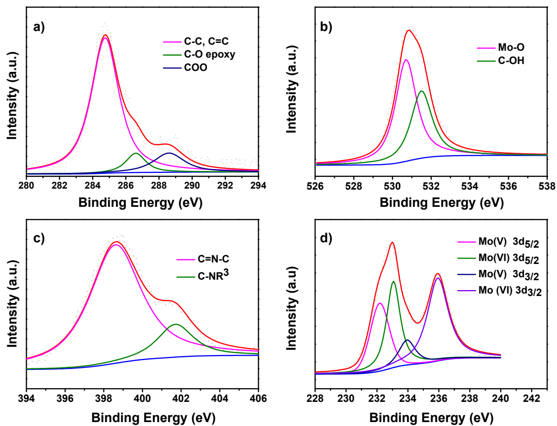
Figure S6: High-resolution (a) C 1s, (b) O 1s, (c) N 1s, and Mo 3d spectra of POM.
