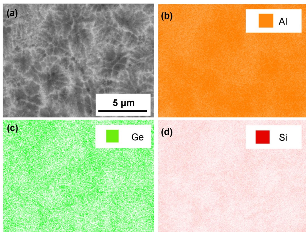
Fig. S1 (a) Back-scattered electron image of the cross-section of Sr-modified \text{Al}_{84.23}\text{Si}_{9.46}\text{Ge}_{6.31} ribbon and corresponding EDS mappings of (b) Al, (c) Ge and (d) Si.
