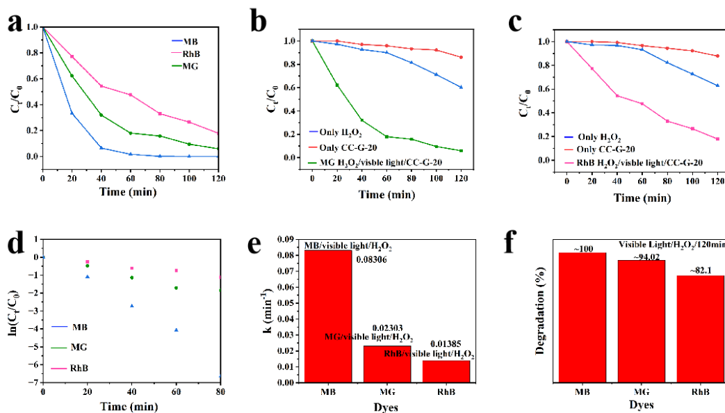
Fig. A1. (a-c) Degradation of dyes under different conditions. (d) \ln(C_t/C_0) of different catalytic systems (CC-G-20/dyes/visible light/ \text{H}_2\text{O}_2 systems) varied with the reaction time. (e) Reaction rate constants of different catalytic systems in A1 (d). (f) Degradation efficiency of different catalytic systems in A1.
