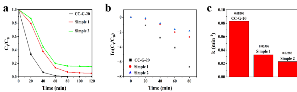
Fig. A2. (a) MB degradation of CC-G-20, simple 1, and simple 2. (b) \ln(C_t/C_0) of CC-G-20, simple 1, and simple 2. Reaction rate constants of three materials in A1 (b).
