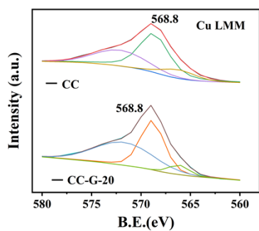
Fig.A4. XPS spectra of CC-G-20 referred to the parent CC. Auger spectrum.
