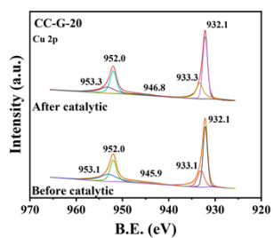
Fig. A5. XPS spectra of CC-G-20. The binding energy of CC-G-20 before and after catalysis.
