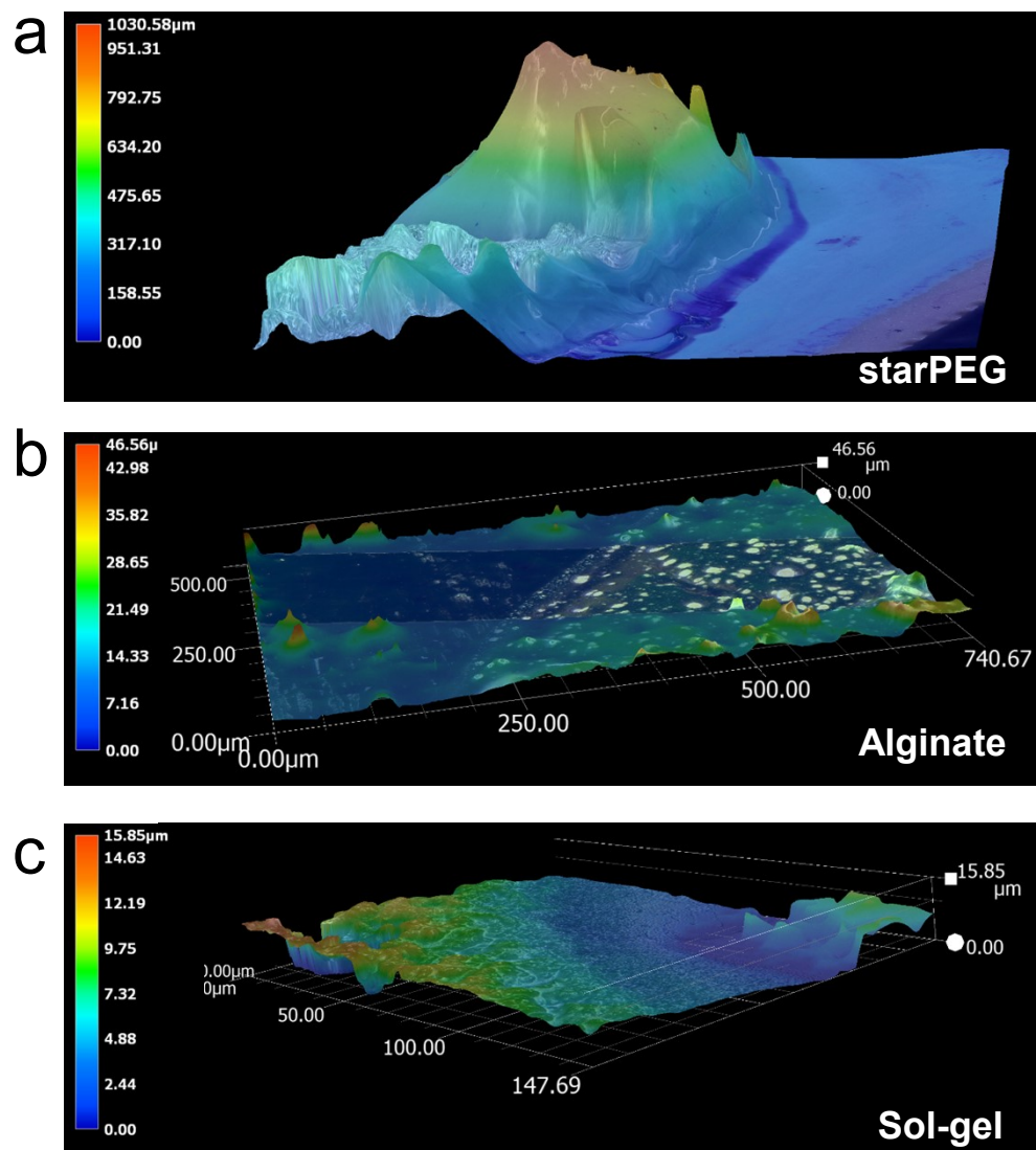
Figure S2. Additional thickness measurements of (a) starPEG-heparin, (b) alginate and (c) sol-gel.
